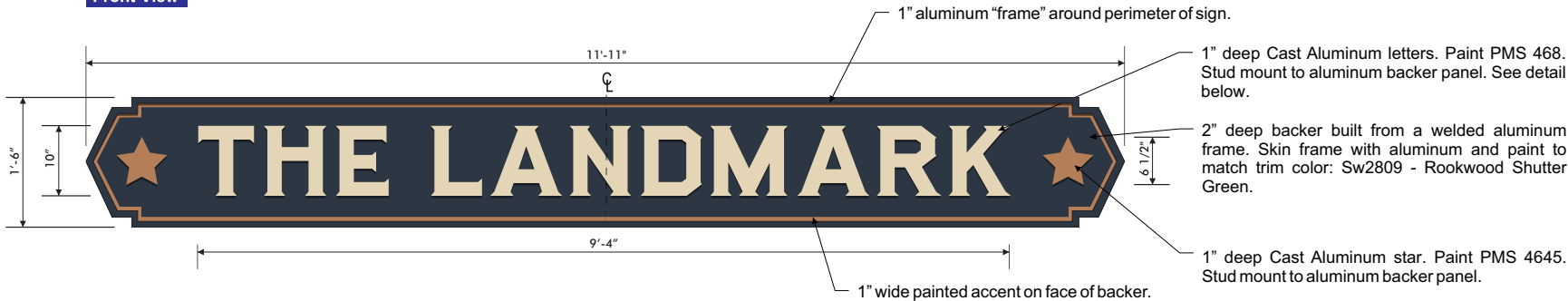
Front View
