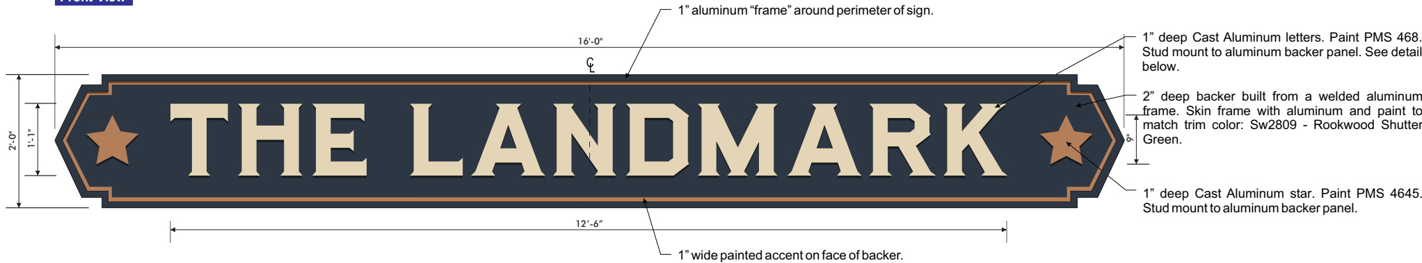
Front View
