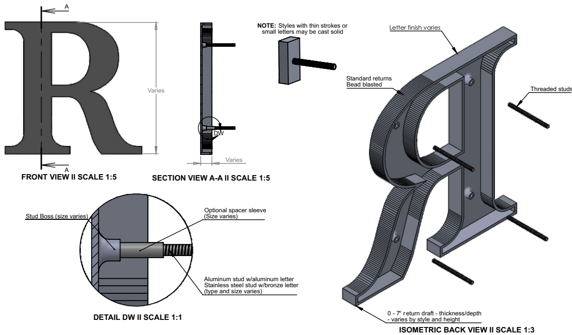
Cast Metal Letter Detail
