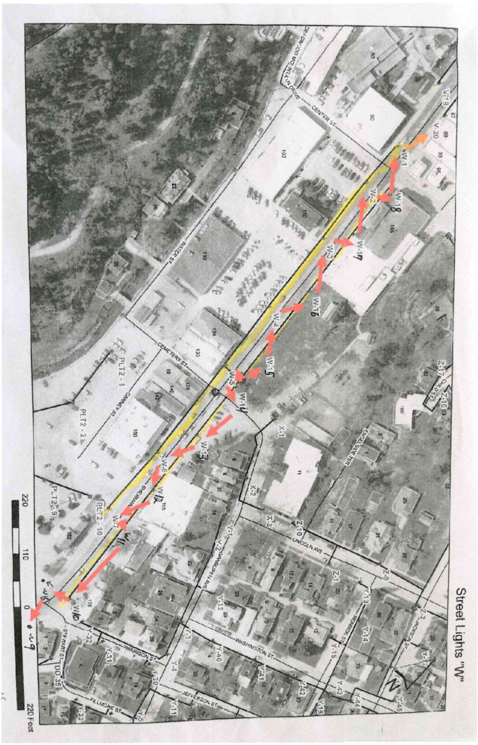
W - 18 Bulbs - 5 APs - 1 Extra AP linking to V
