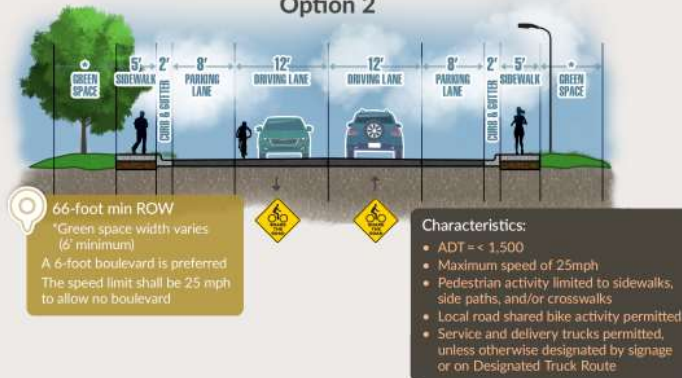
Figure 10-7. Urban Local Option 2
