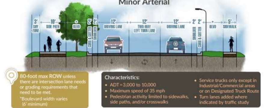
Figure 10-3. Urban Minor Arterial
