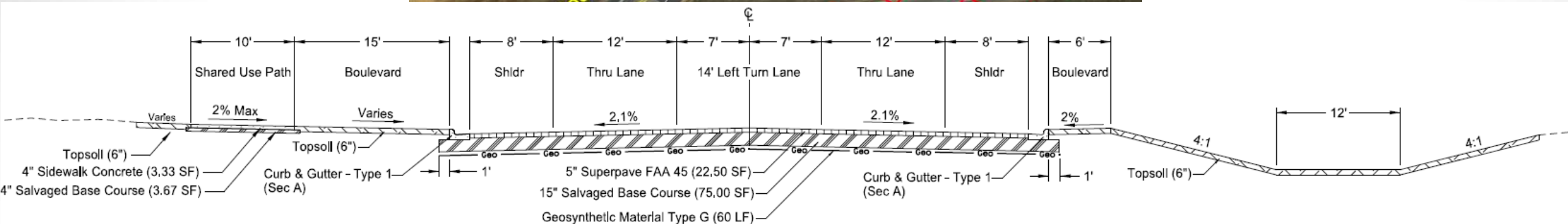
Proposed Typical Section 1 - West Business Loop
