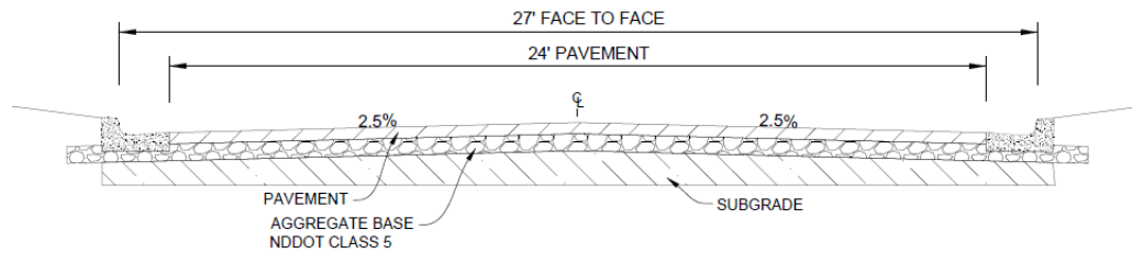
Figure 1: Private Access Road Typical Section
