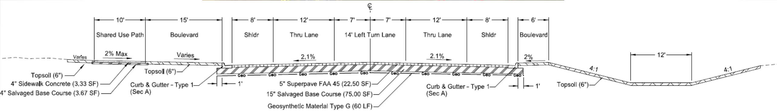
Proposed Typical Section 1 - West Business Loop Sta 186+75 to Sta 232+40 Sta 241+16 to Sta 255+50
