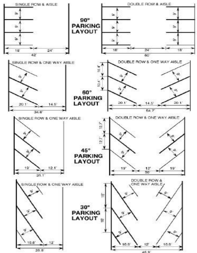
Figure 7.1: Parking Aisle and Space
