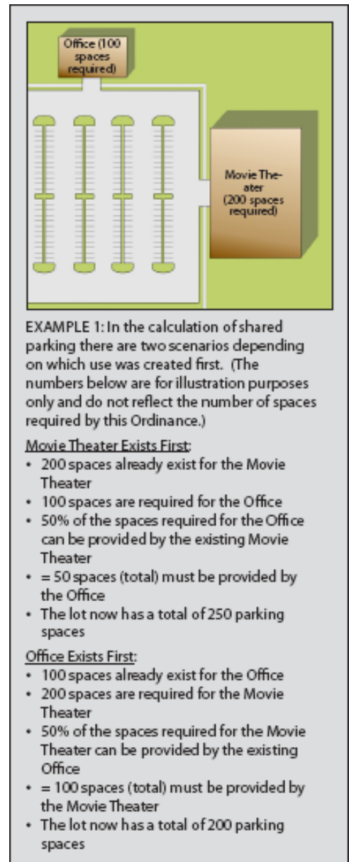
Figure 7.2: Parking Calculation Example
