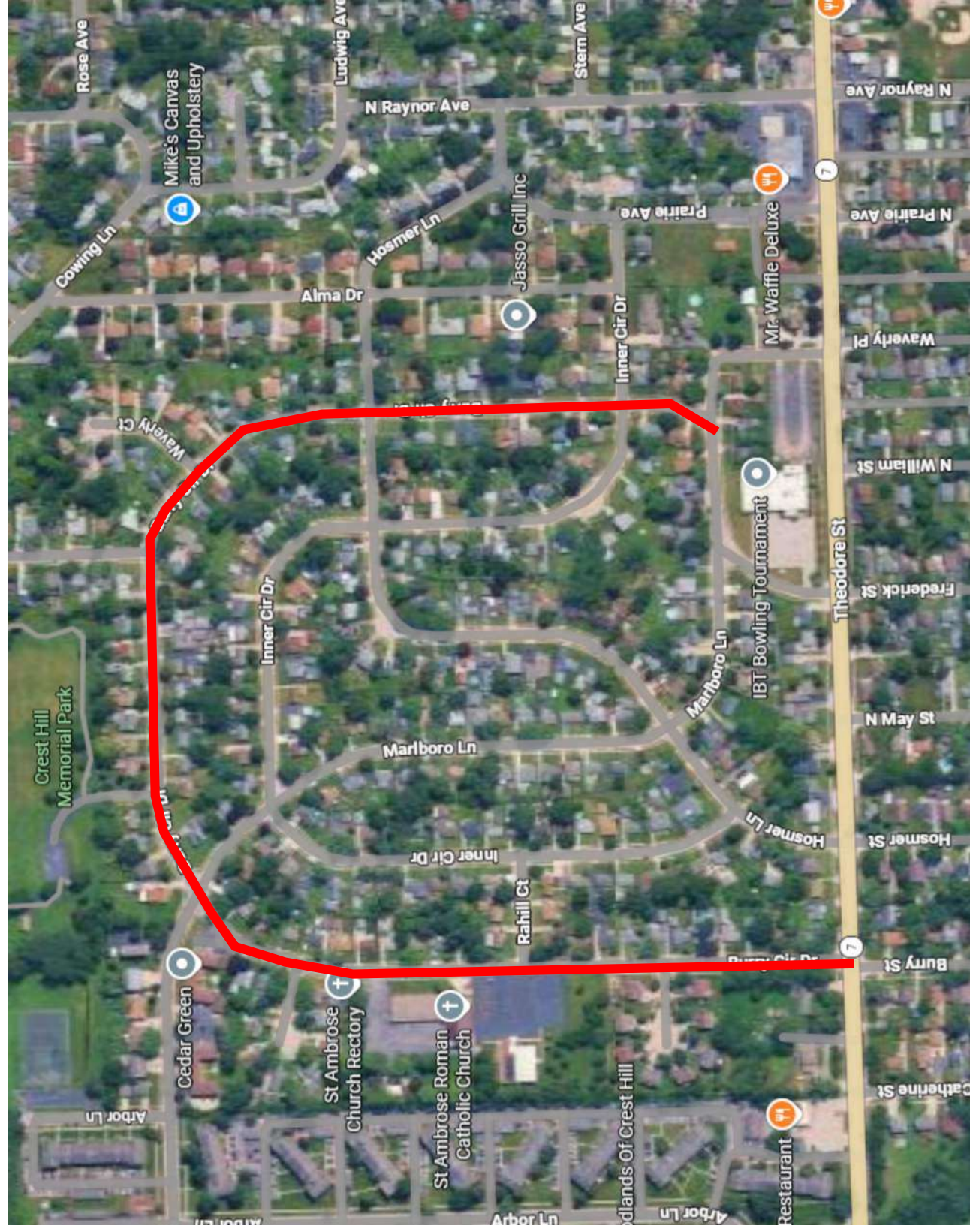
Burry Circle Drive Watermain Replacement Limits Map
