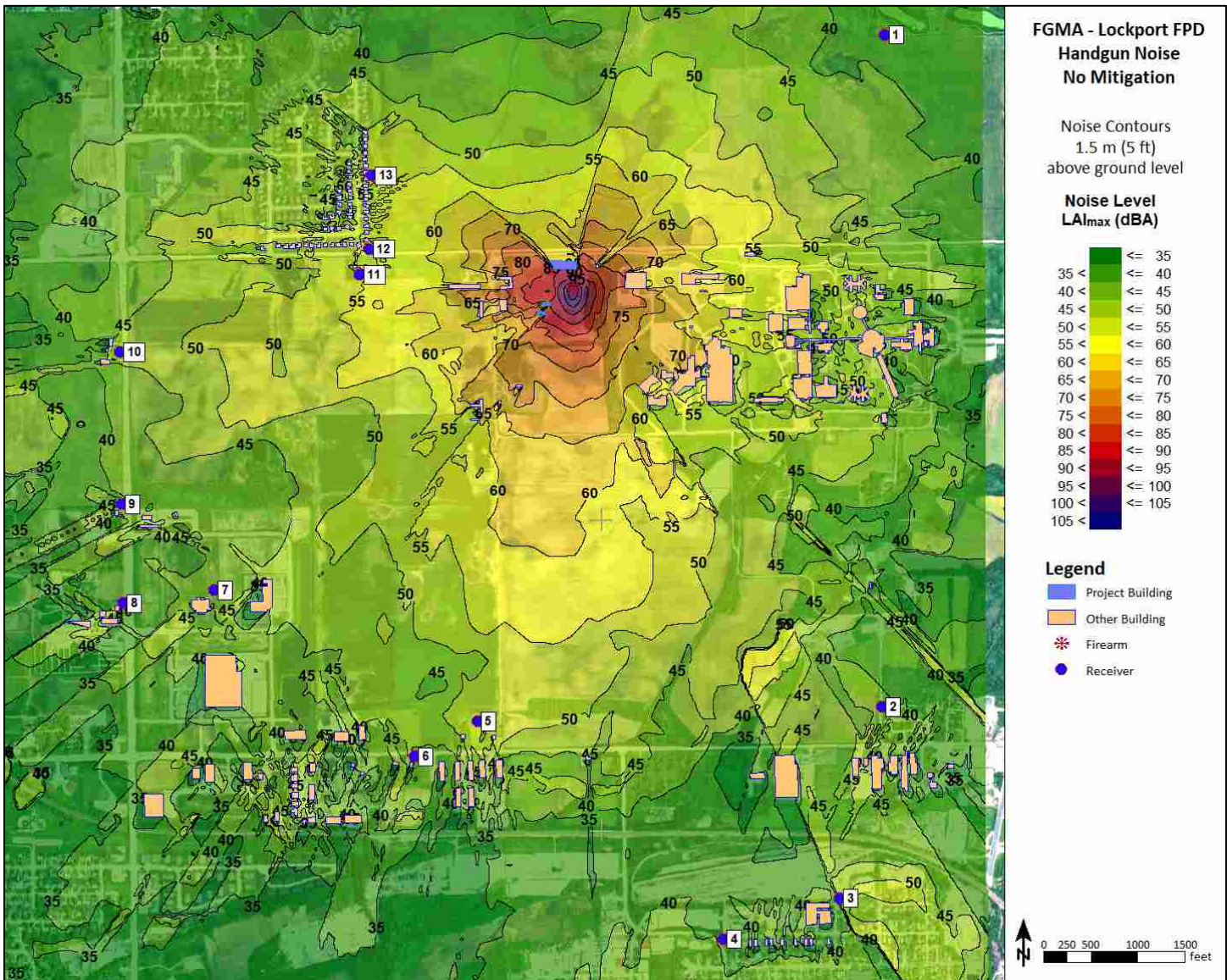
Figure 8: Noise Contour Map of Predicted Handgun Noise Transmission to Surrounding Areas, Without Mitigation
