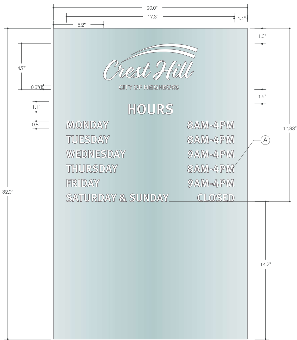
Type P3 Vinyl Overall Size 17.36"w x 16.25"h
