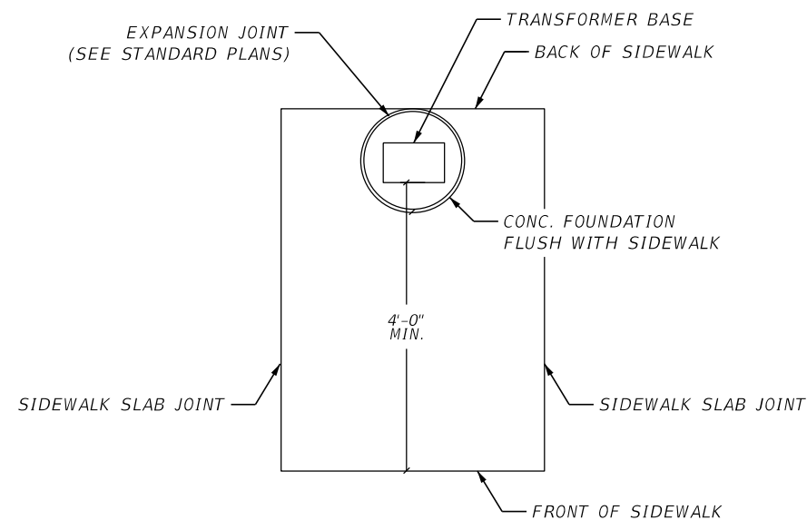
LIGHT POLE INSTALLATION DETAIL ON SIDEWALK (N.T.S)
