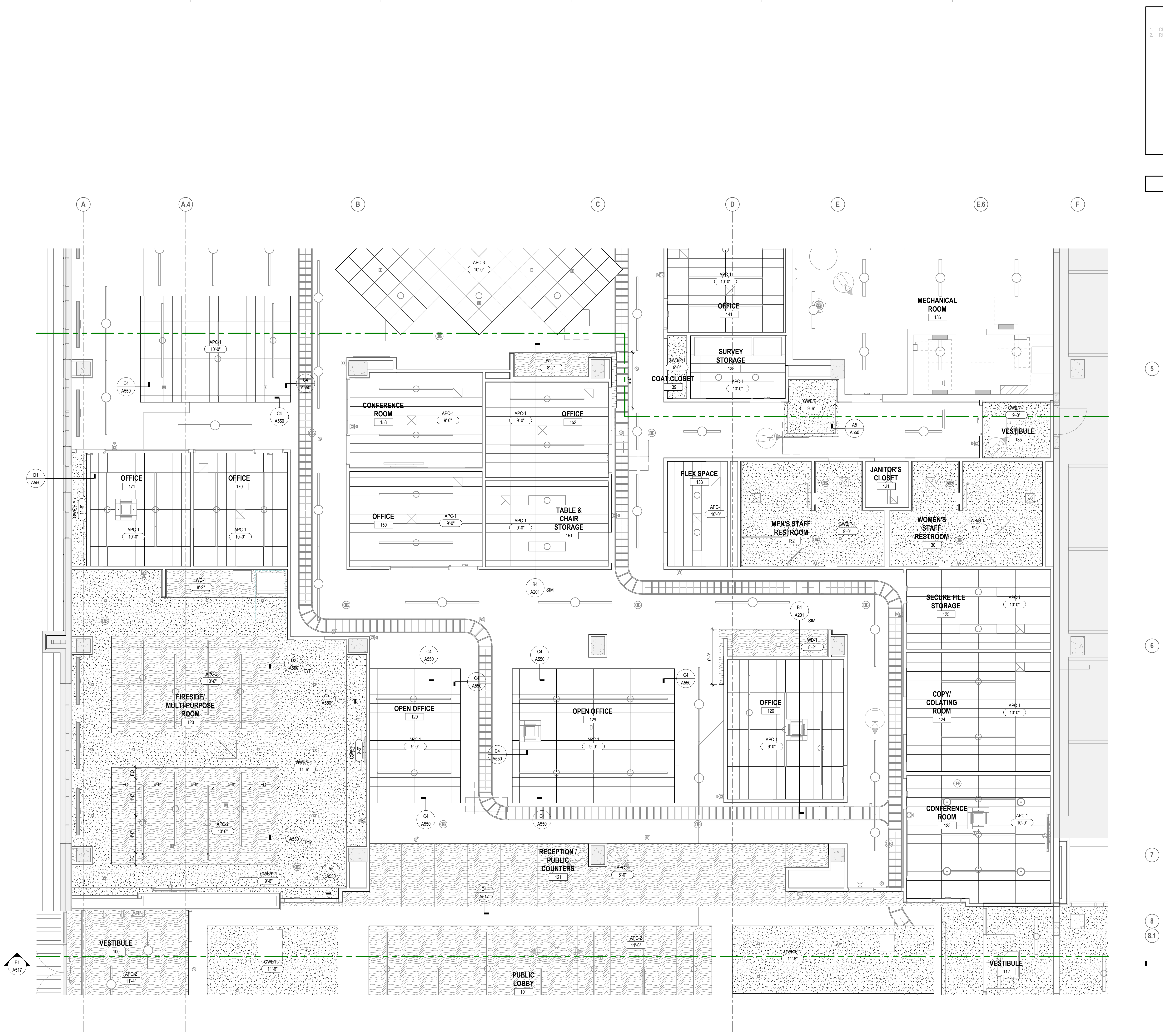
A1 CEILING PLAN LEVEL 1 AREA B SCALE: 1/4" = 1'-0"
