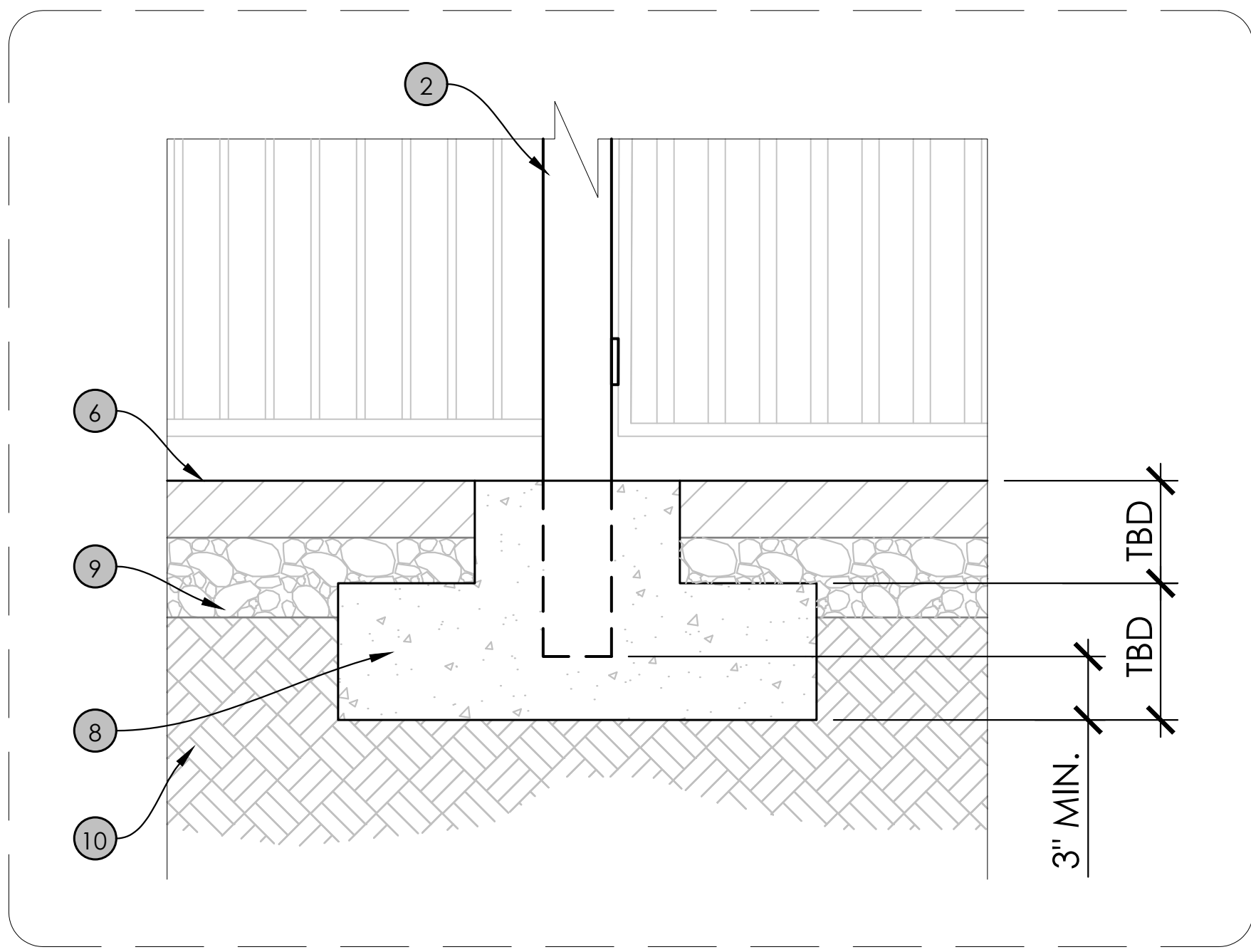
A.2 POST FOOTING ENLARGEMENT
