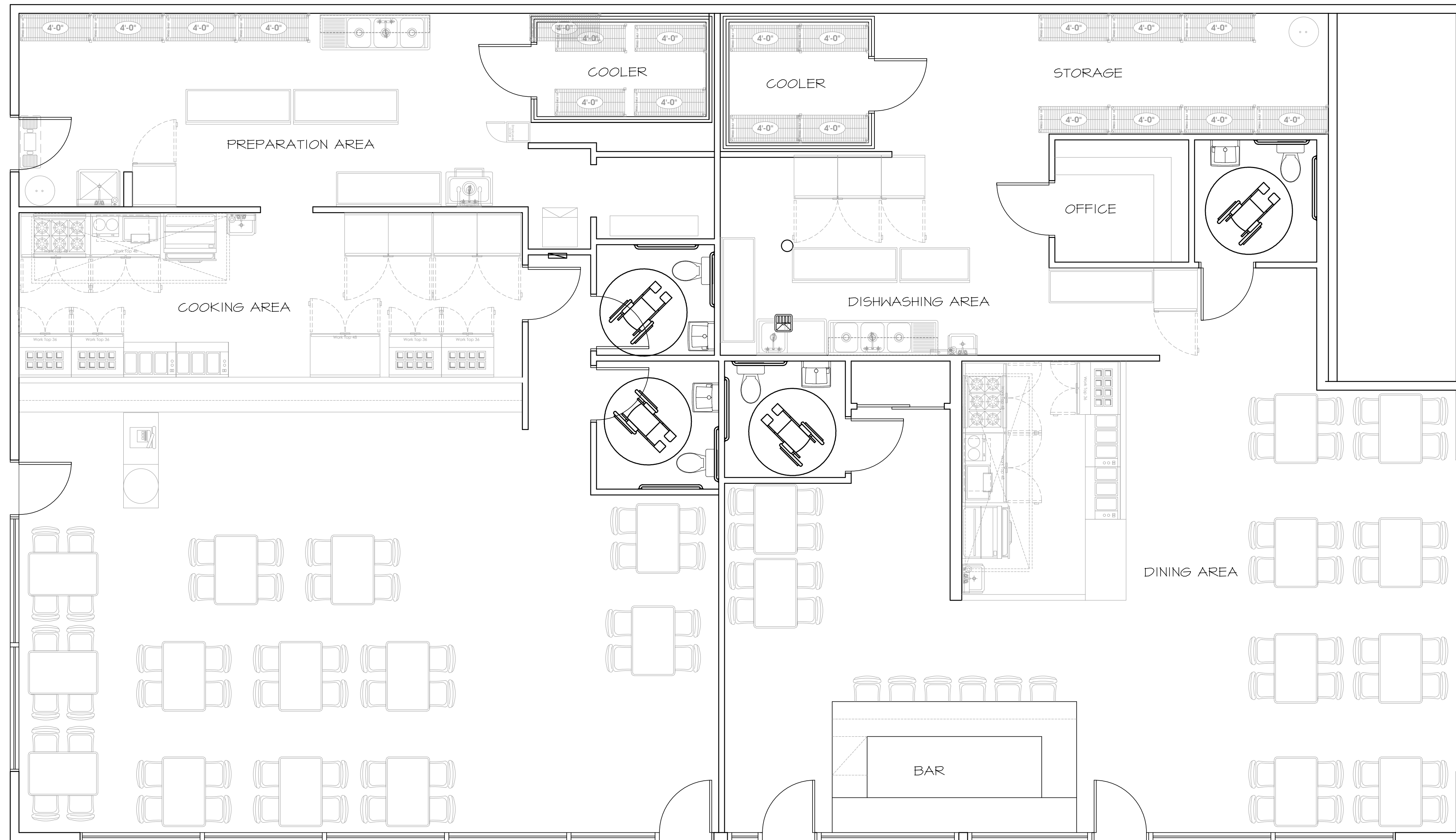
EXISTING FLOOR PLAN AREA 2 RESTAURANT, COACHELLA , CA
