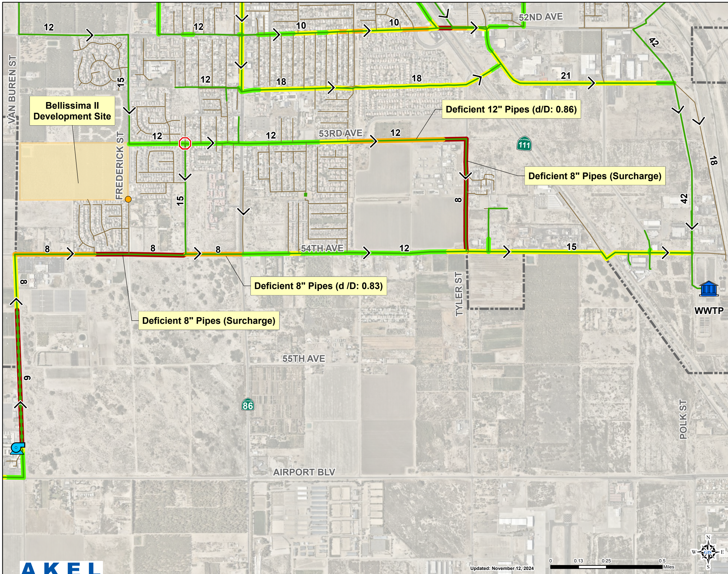
Figure 2 Existing System + Bellissima II Capacity Evaluation Sewer Capacity Analysis City of Coachella
