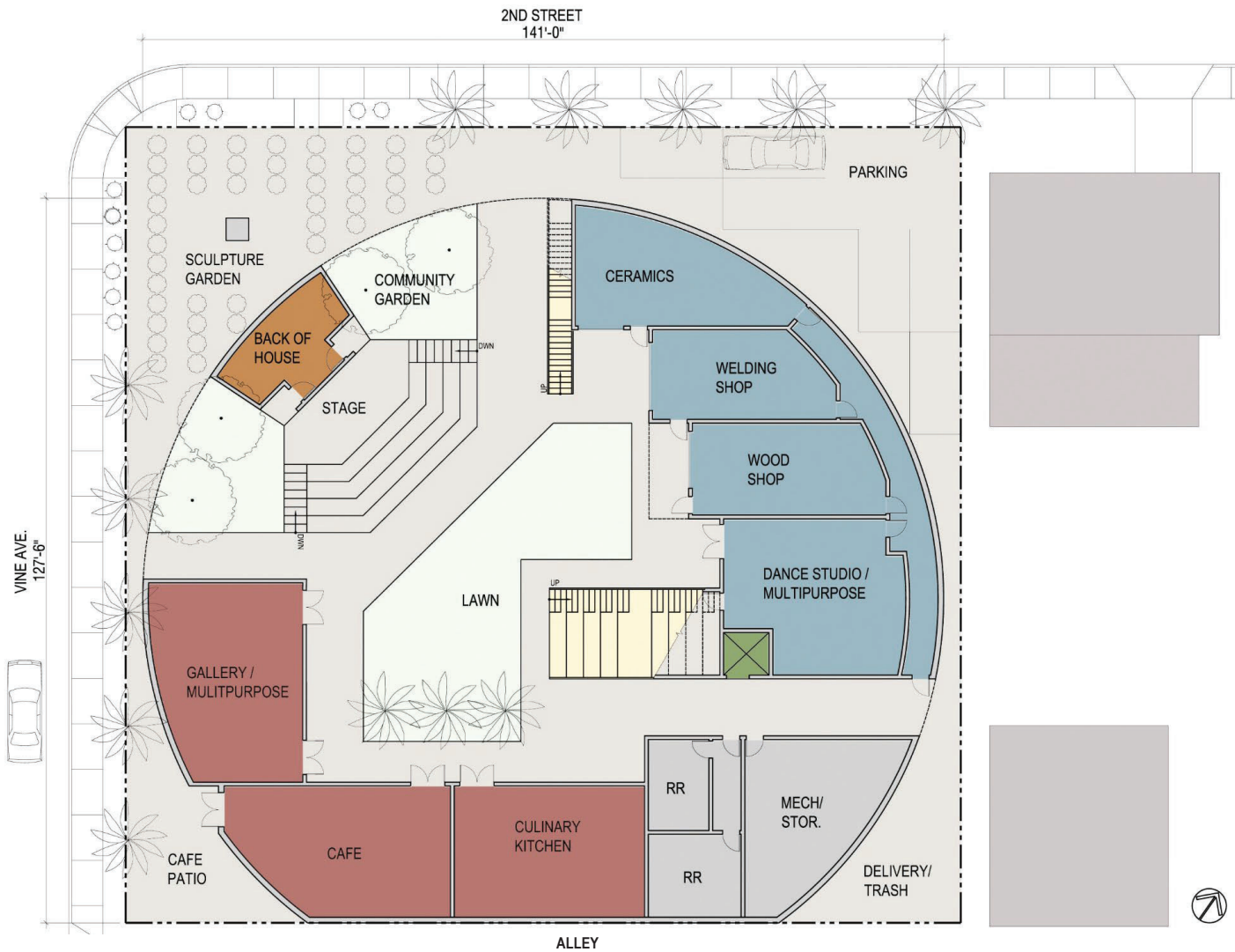
SITE PLAN: Option 2 – First Floor
