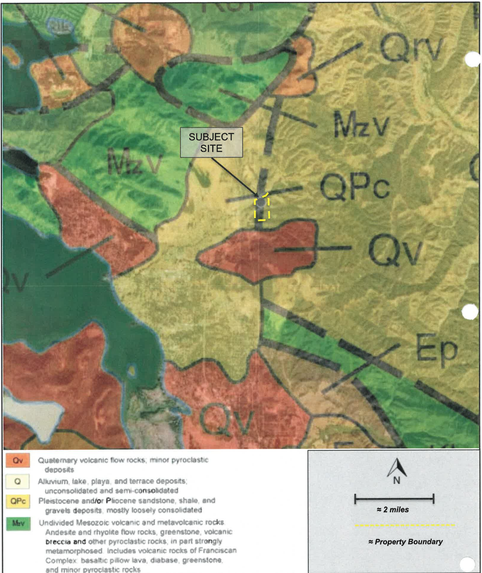
FIGURE 2: SITE GEOLOGY
