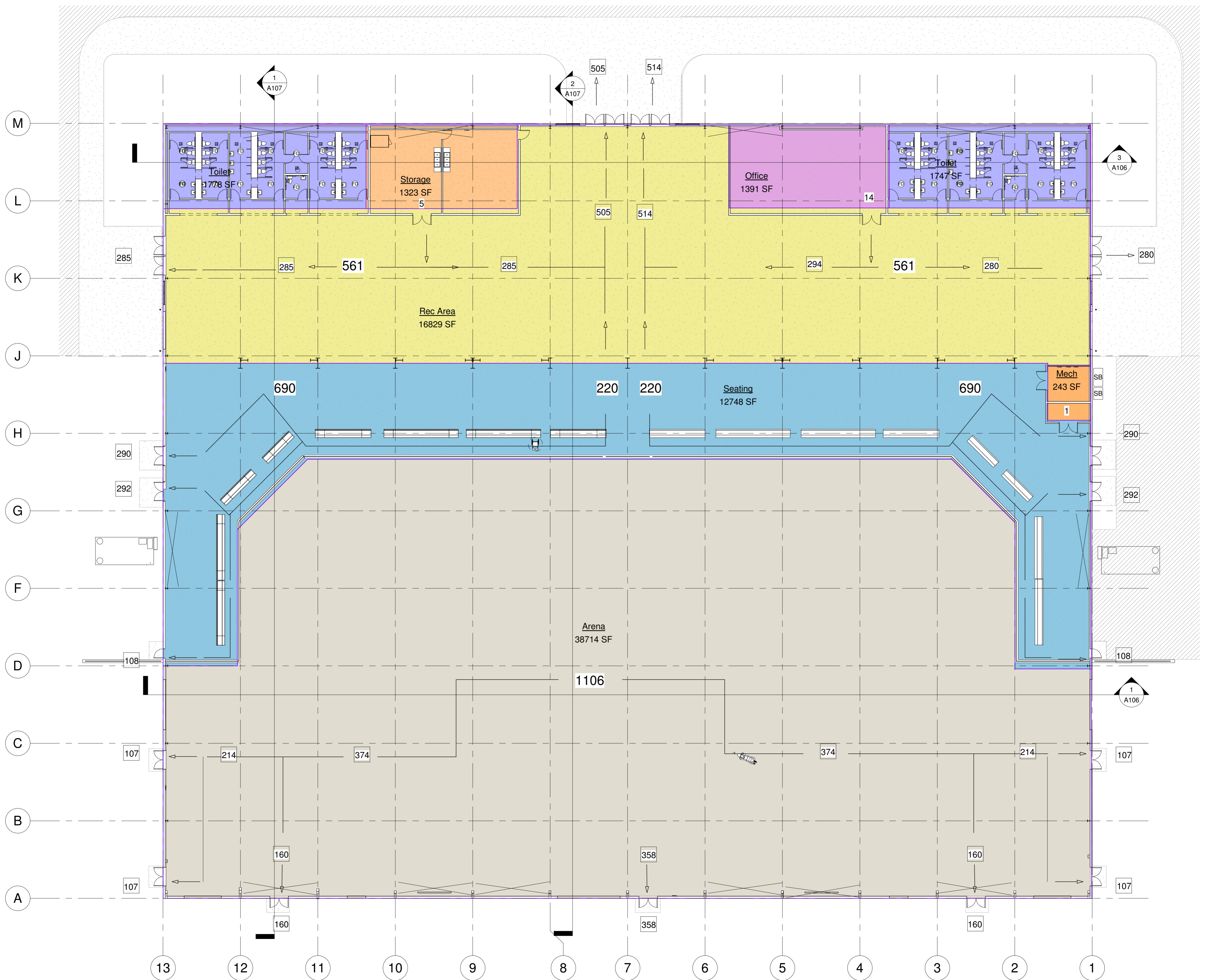
① Level 1 Exit Plan 1/16" = 1'-0"
