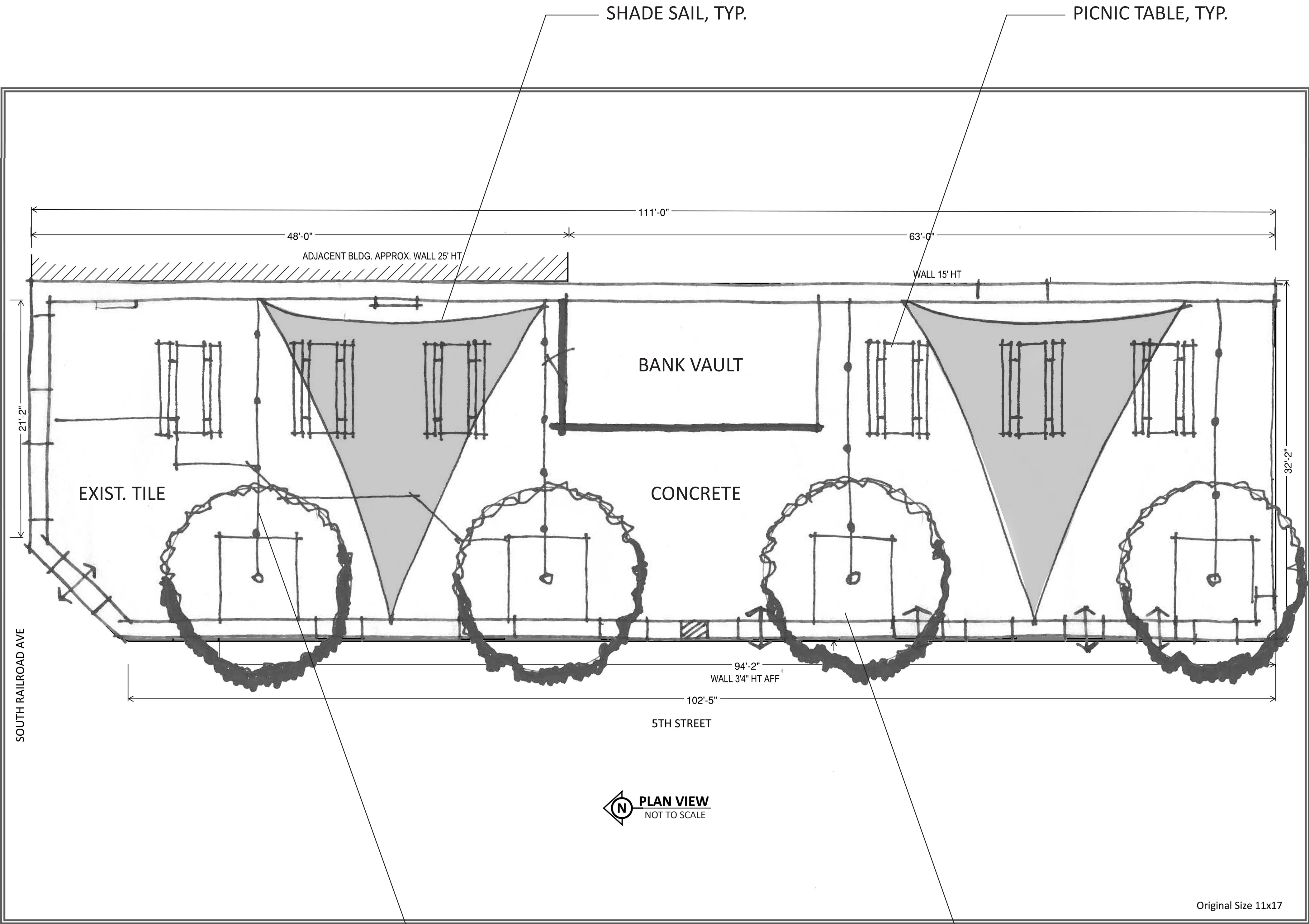
CONCRETE CUTOUT
