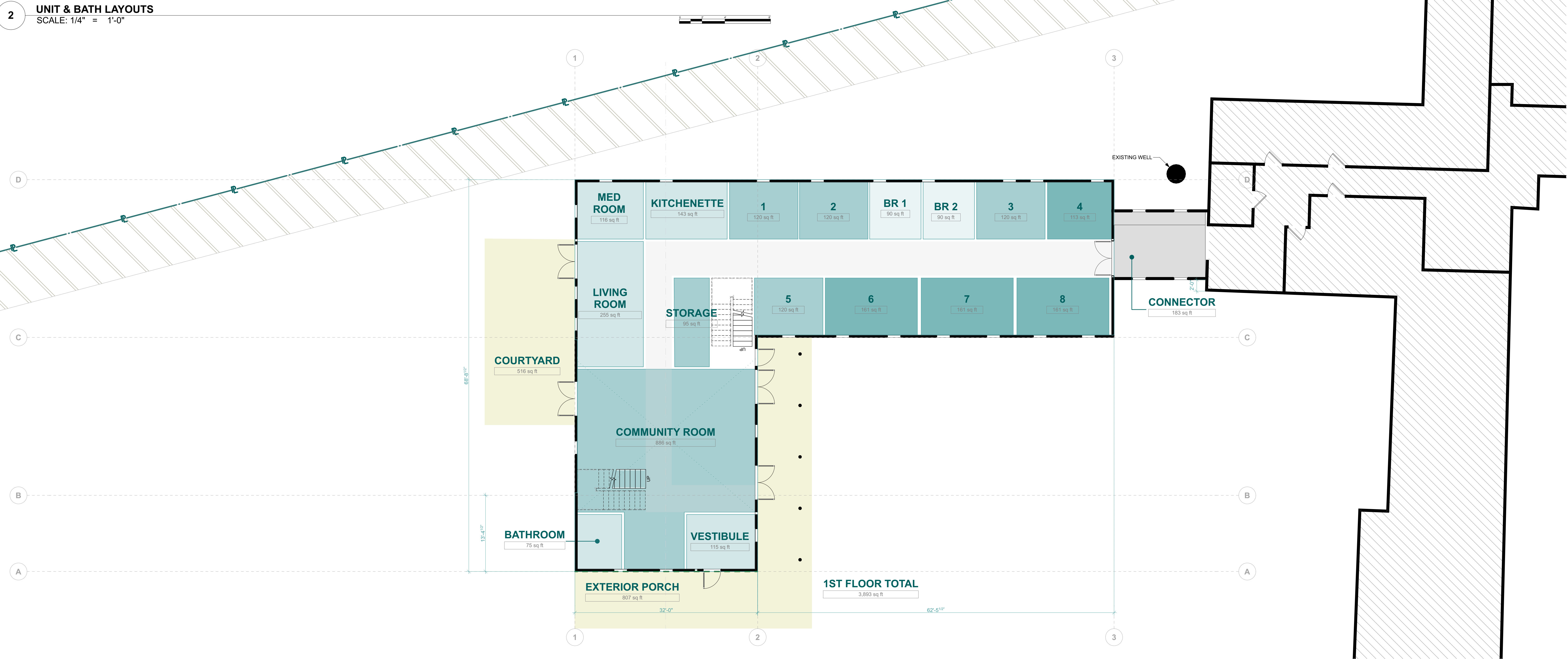
1 1ST FLOOR PLAN SCALE: 1/8" = 1'-0"
