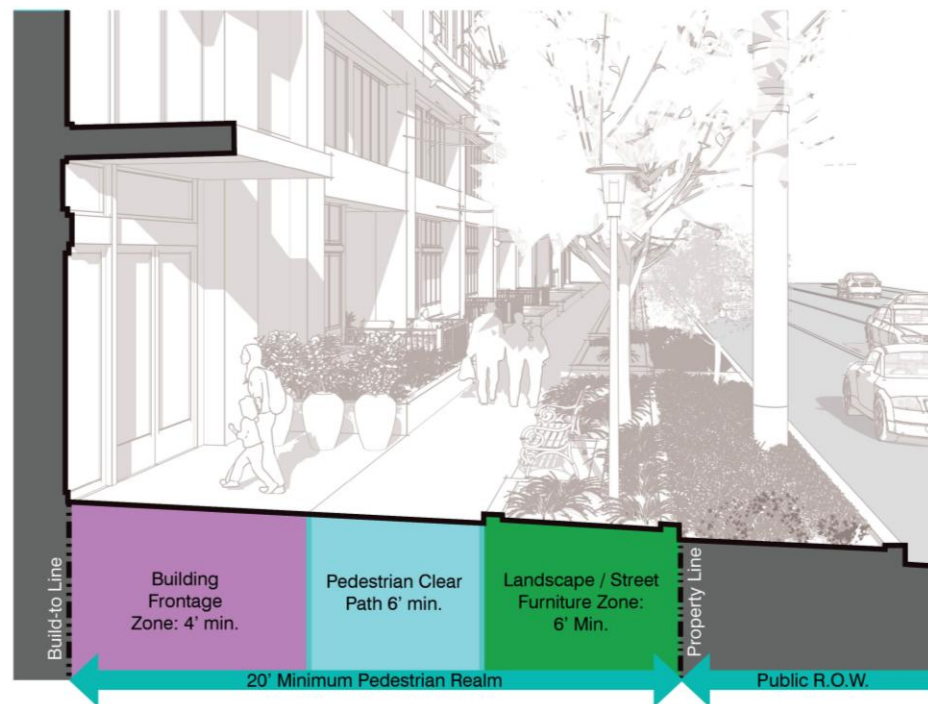
Figure 17.57-4: Perimeter Street Pedestrian Realm
