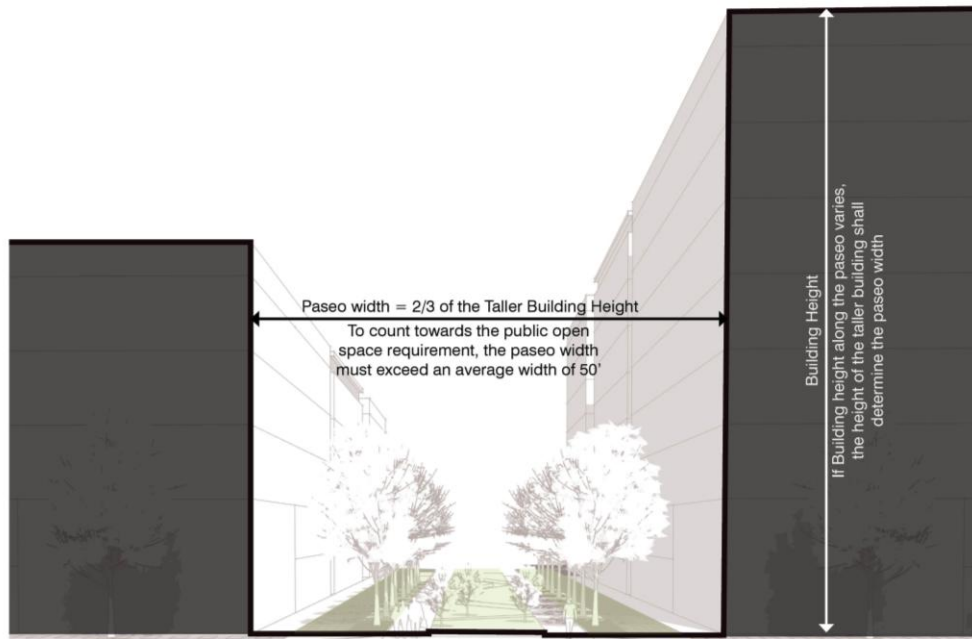
Figure 17.57-5: Paseo Width
