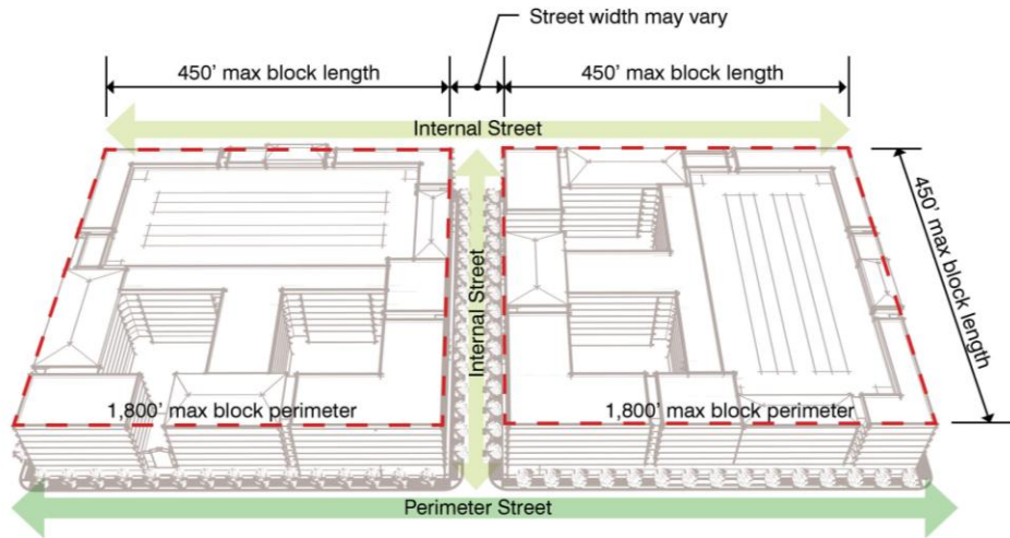
Figure 17.57-2: Maximum Block Length
