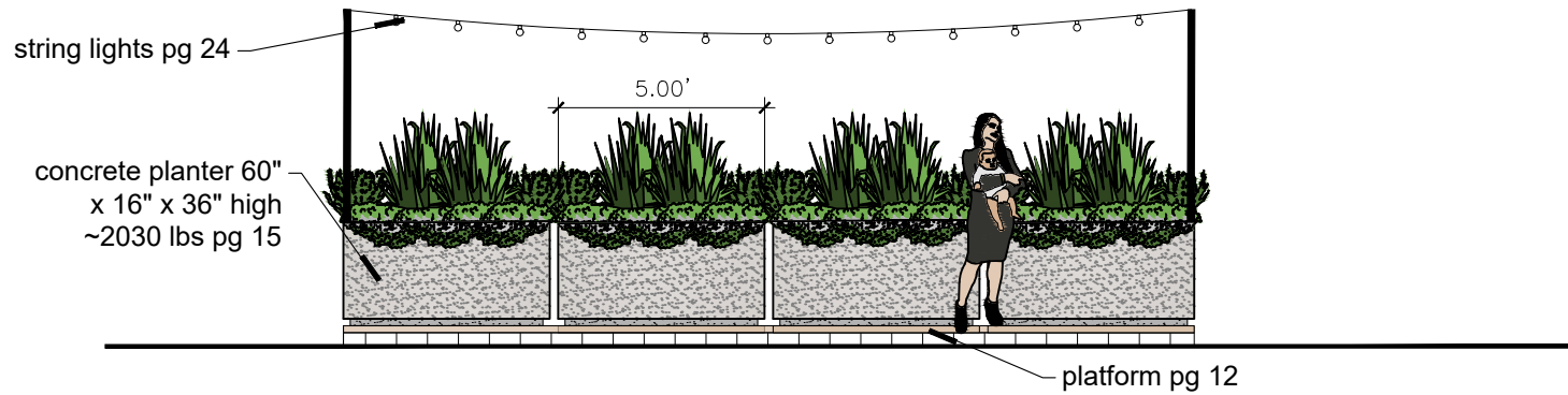
PLANTERS only (no railing) - elevation
