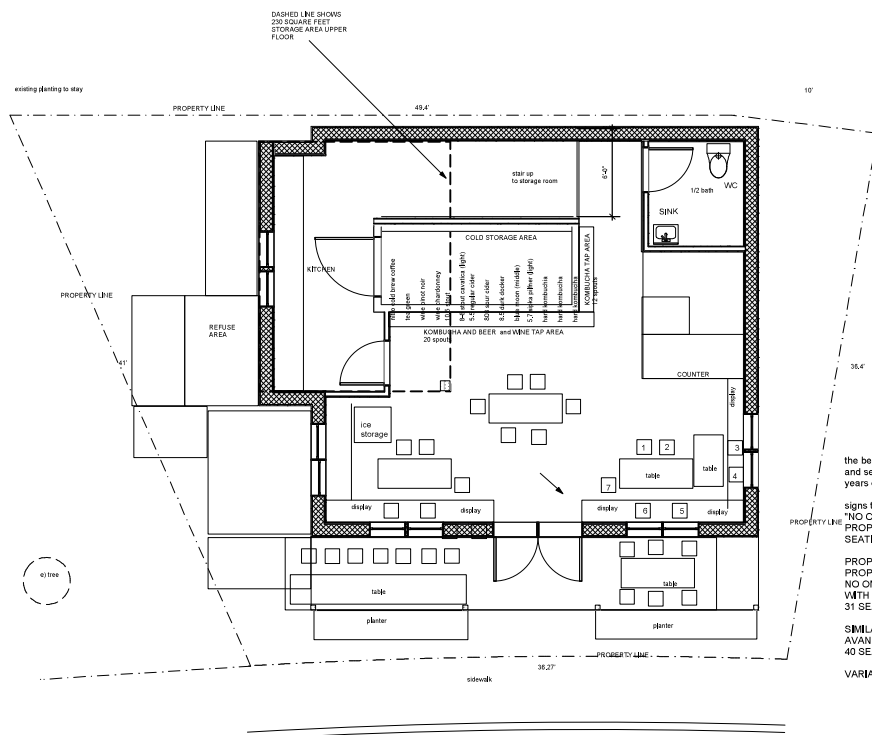
SITE PLAN 1/4" = 1' 0"
