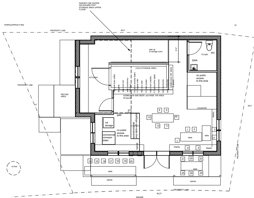
SITE PLAN 1/4" = 1' 0"
