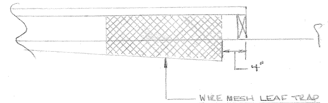
ENLARGED SECTION D
