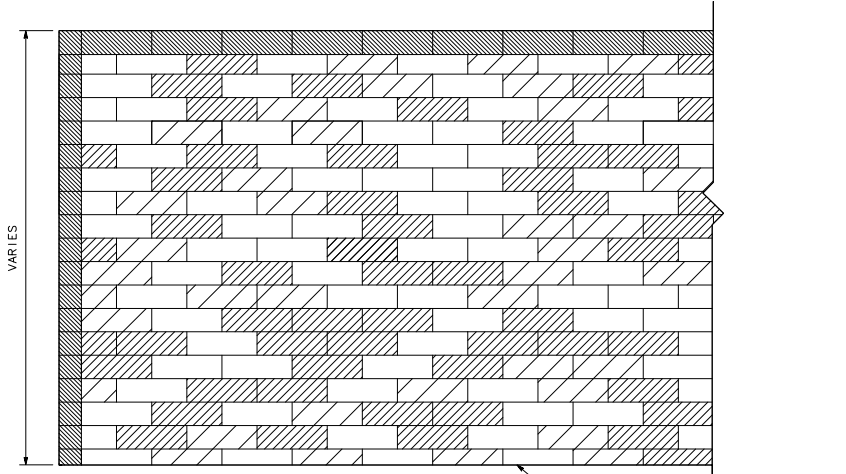
END WALL CONDITION NO SCALE
