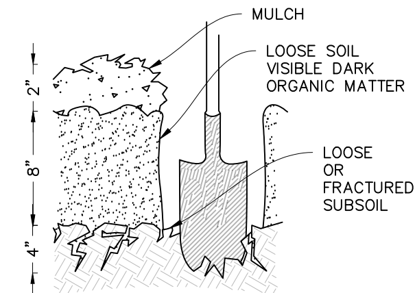
BMP T5.13 SOIL QUALITY AND DEPTH NOT TO SCALE
