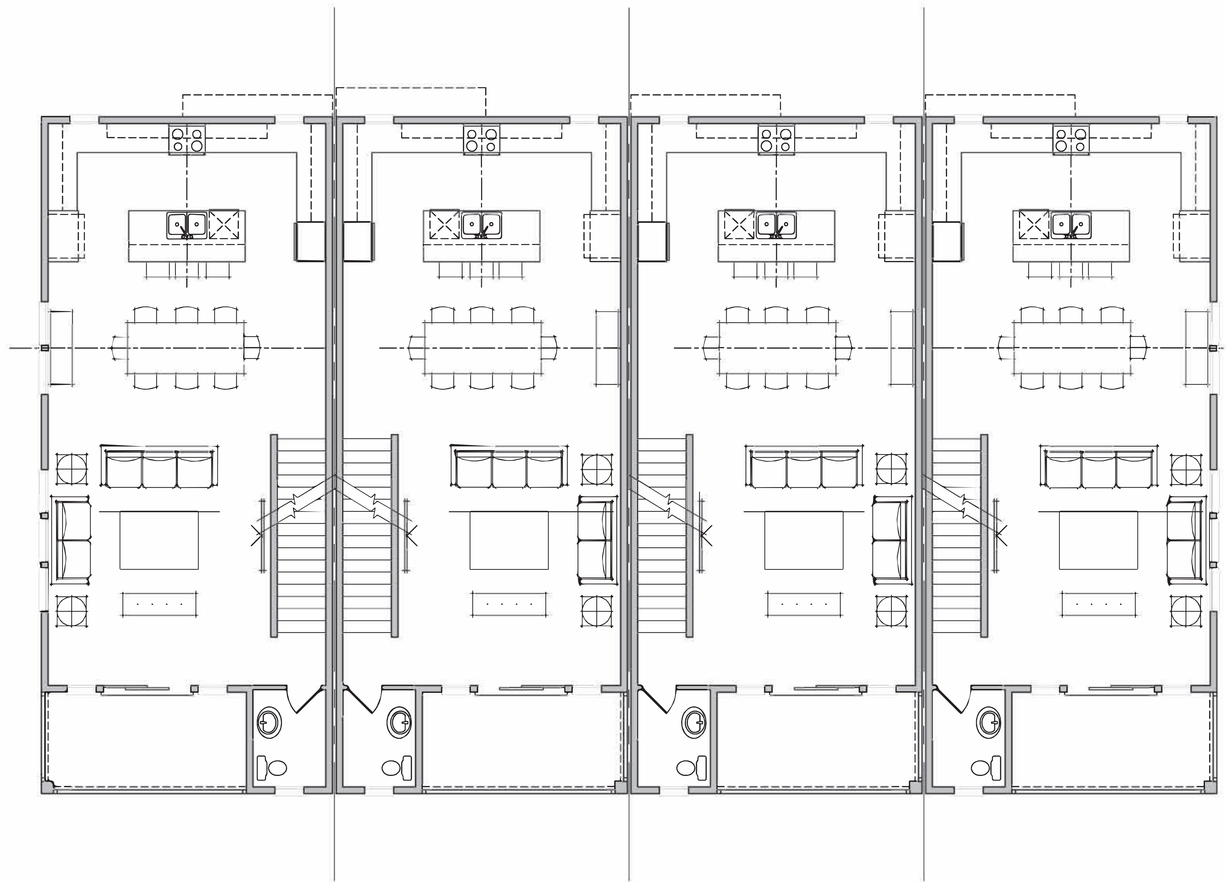
PLAN 3-R
