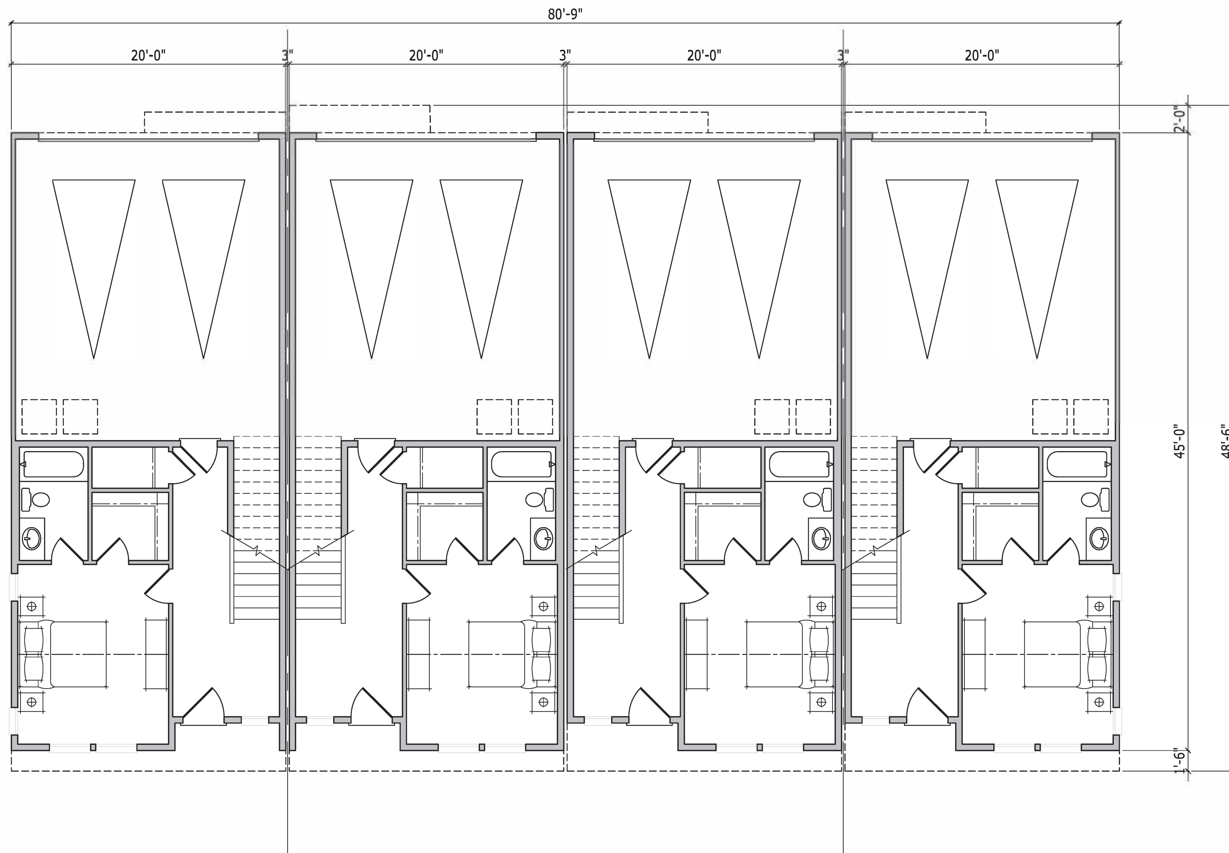
PLAN 3-R
