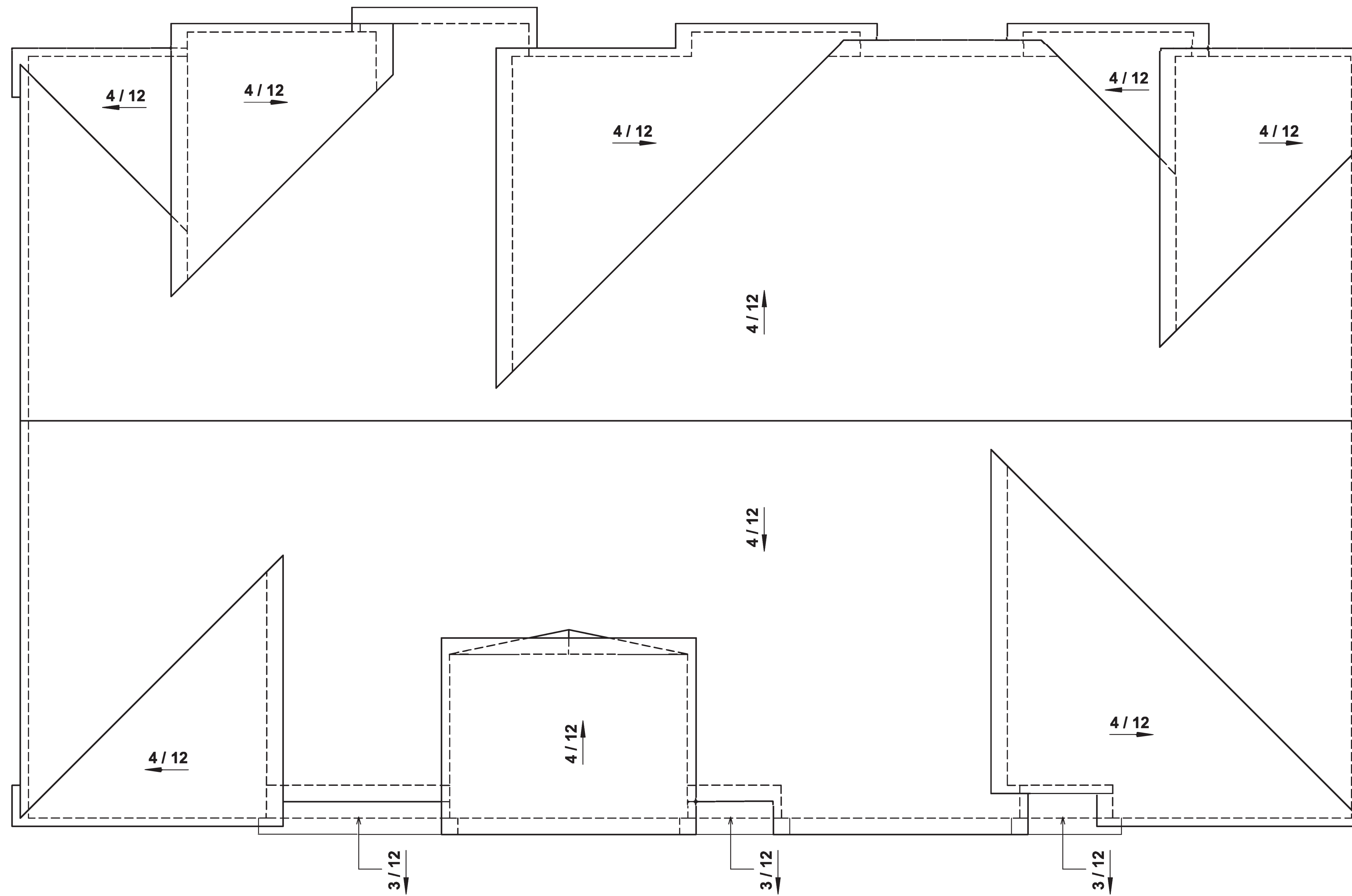
ROOF PLAN
