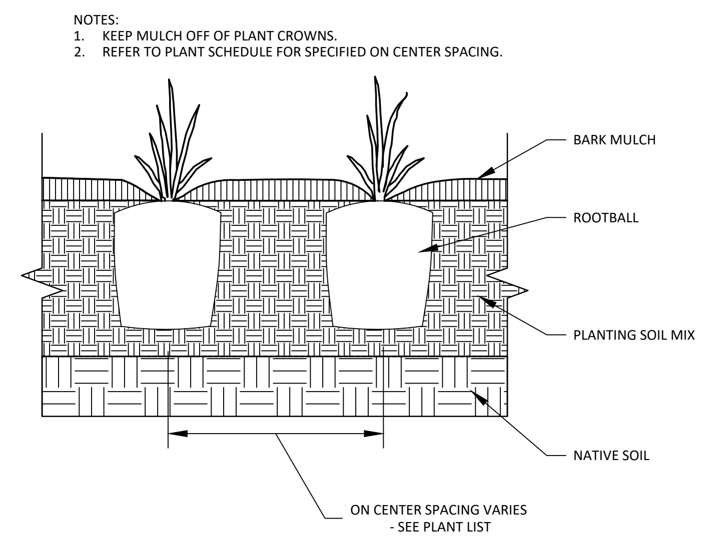
4 GROUNDCOVER PLANTING NTS
