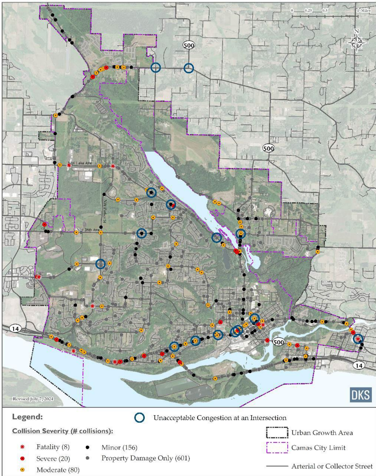
FIGURE 16: STREET NETWORK CONGESTION AND SAFETY
