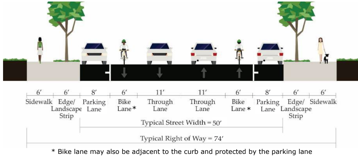
FIGURE 23: TYPICAL CROSS-SECTION FOR RESIDENTIAL COLLECTOR STREET
