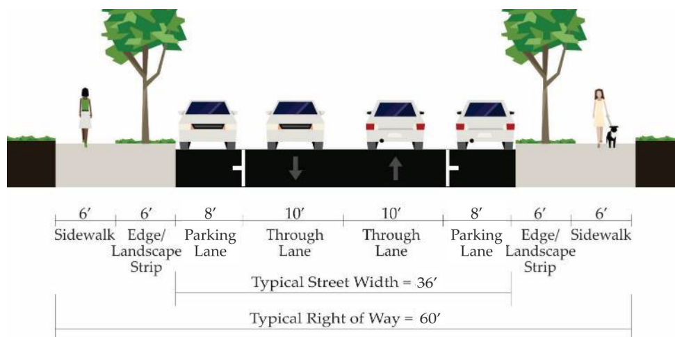
FIGURE 27: TYPICAL CROSS-SECTION FOR COMMERCIAL OR INDUSTRIAL LOCAL STREET
