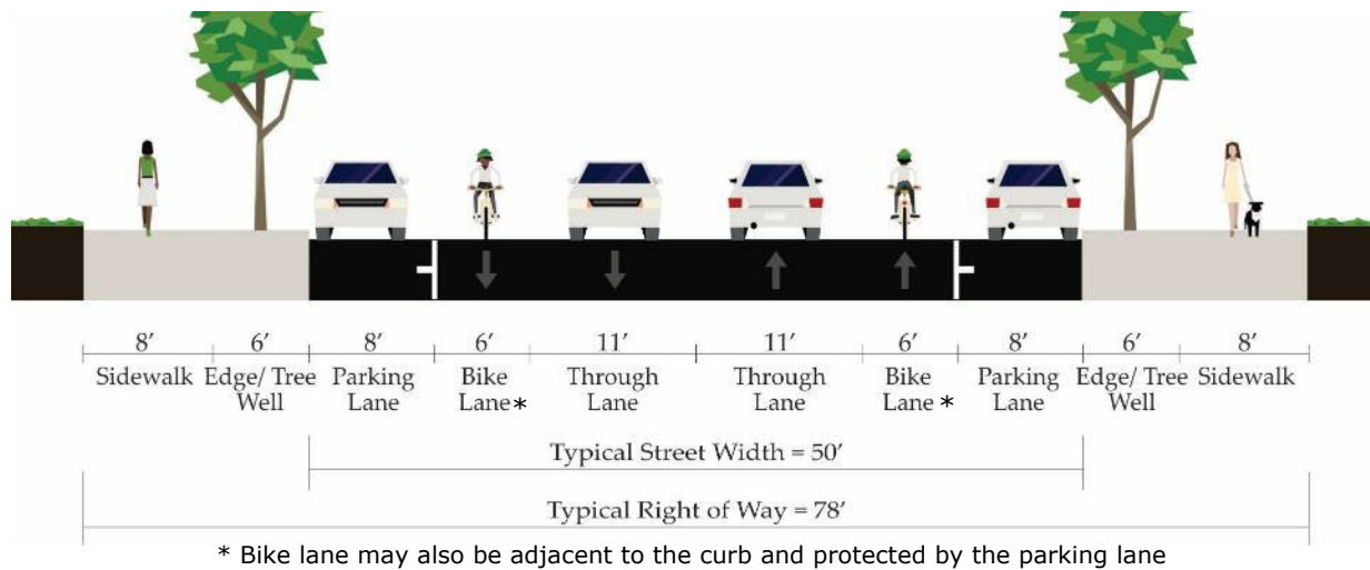
FIGURE 22: TYPICAL CROSS-SECTION FOR MIXED-USE COLLECTOR STREET
