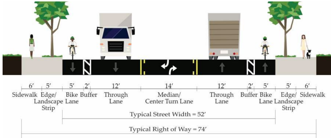
FIGURE 21: TYPICAL CROSS-SECTION FOR COMMERCIAL OR INDUSTRIAL ARTERIAL STREET
