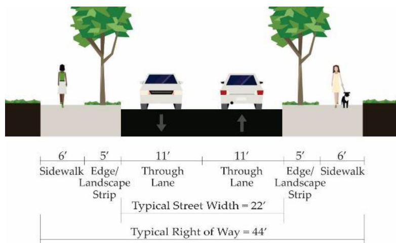
FIGURE 27: TYPICAL CROSS-SECTION FOR COMMERCIAL OR INDUSTRIAL LOCAL STREET
