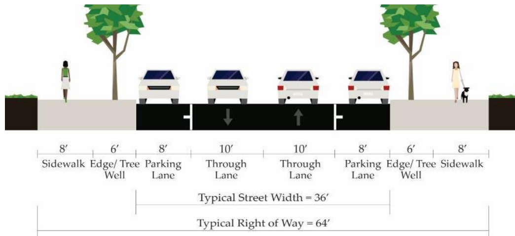
FIGURE 26: TYPICAL CROSS-SECTION FOR RESIDENTIAL LOCAL STREET
