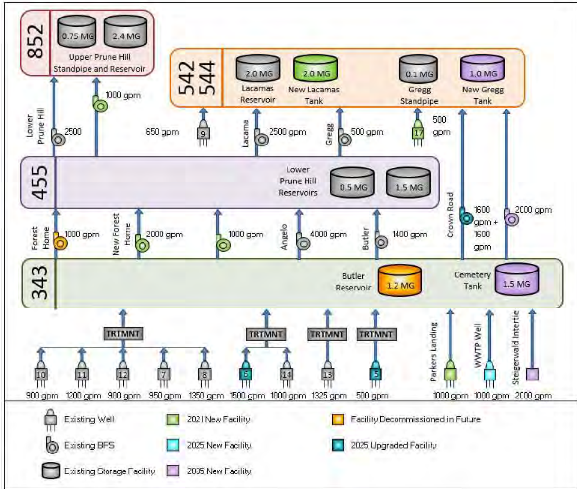
Figure 9.7 Recommended Supply, Pumping, and Storage Improvements
