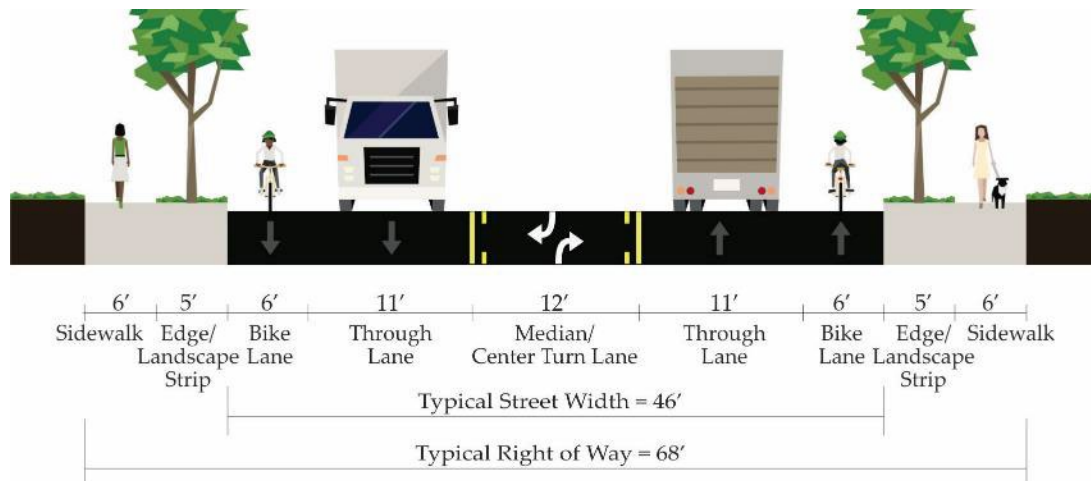
FIGURE 24: TYPICAL CROSS-SECTION FOR COMMERCIAL OR INDUSTRIAL COLLECTOR STREET
