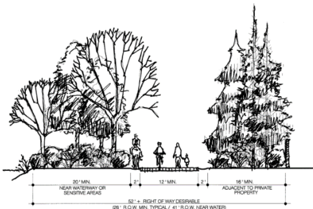
FIGURE 29: TYPICAL DESIGN FOR REGIONAL SHARED-USE PATHS
