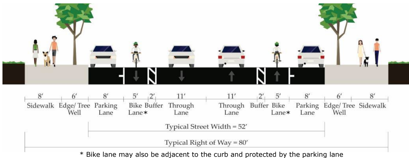
FIGURE 19: TYPICAL CROSS-SECTION FOR MIXED-USE ARTERIAL STREET
