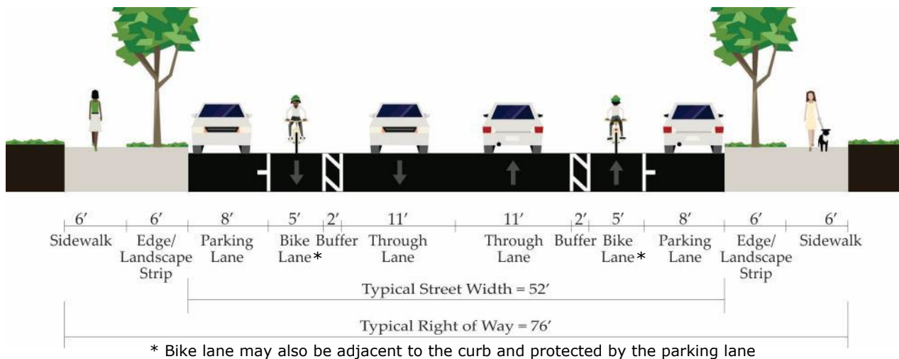
FIGURE 20: TYPICAL CROSS-SECTION FOR RESIDENTIAL ARTERIAL STREET
