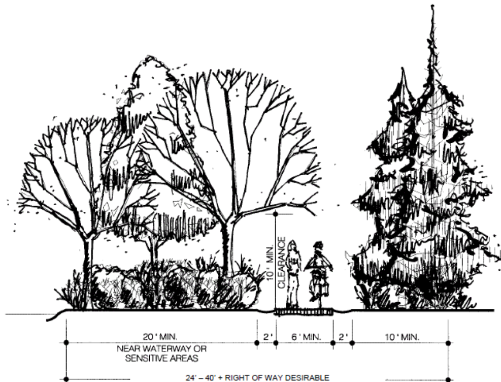
FIGURE 30: TYPICAL DESIGN FOR LOCAL SHARED-USE PATHS
