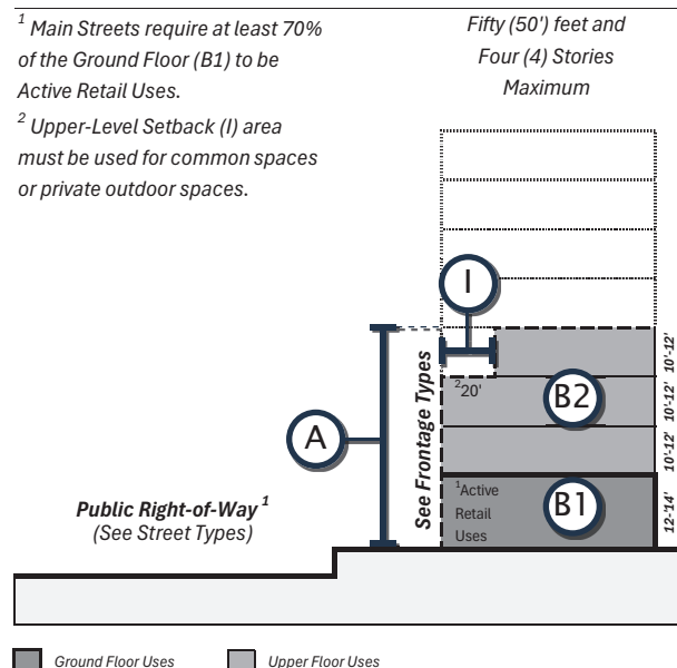
Figure 16. Height and Use Diagram (A-B)
