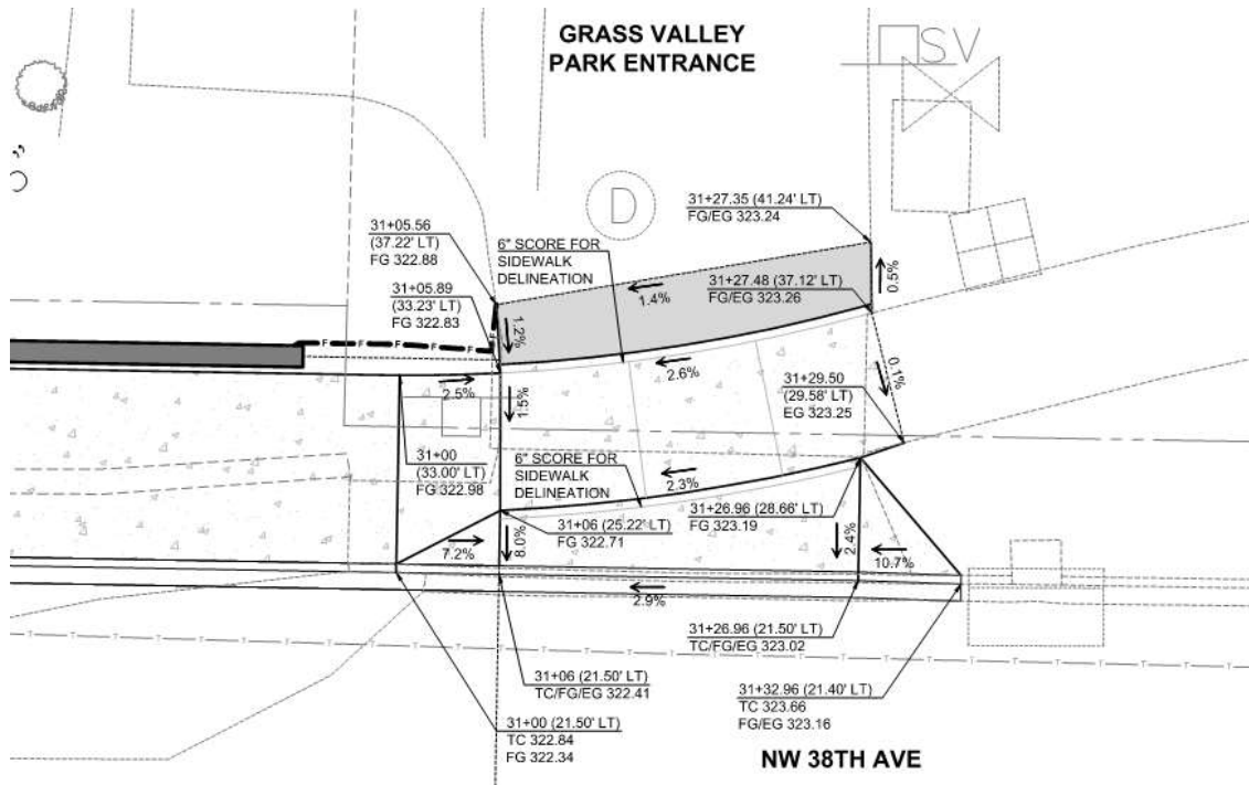
Grass Valley Park driveway grading exhibit
