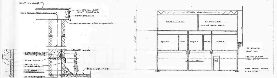
SECTION A
