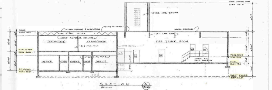
SECTION A
