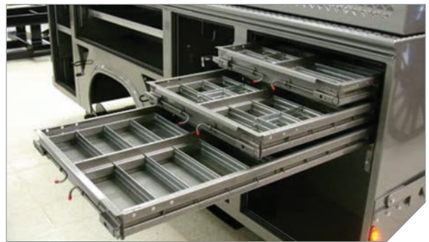
THREE-DRAWER UNIT
