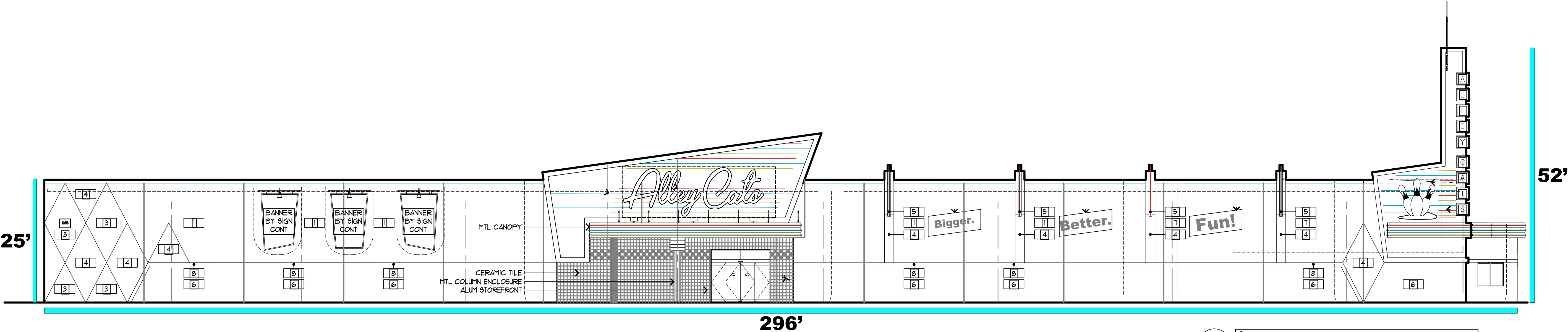
D SOUTH ELEVATION A201 SCALE: 3/32" = 1'-0"
