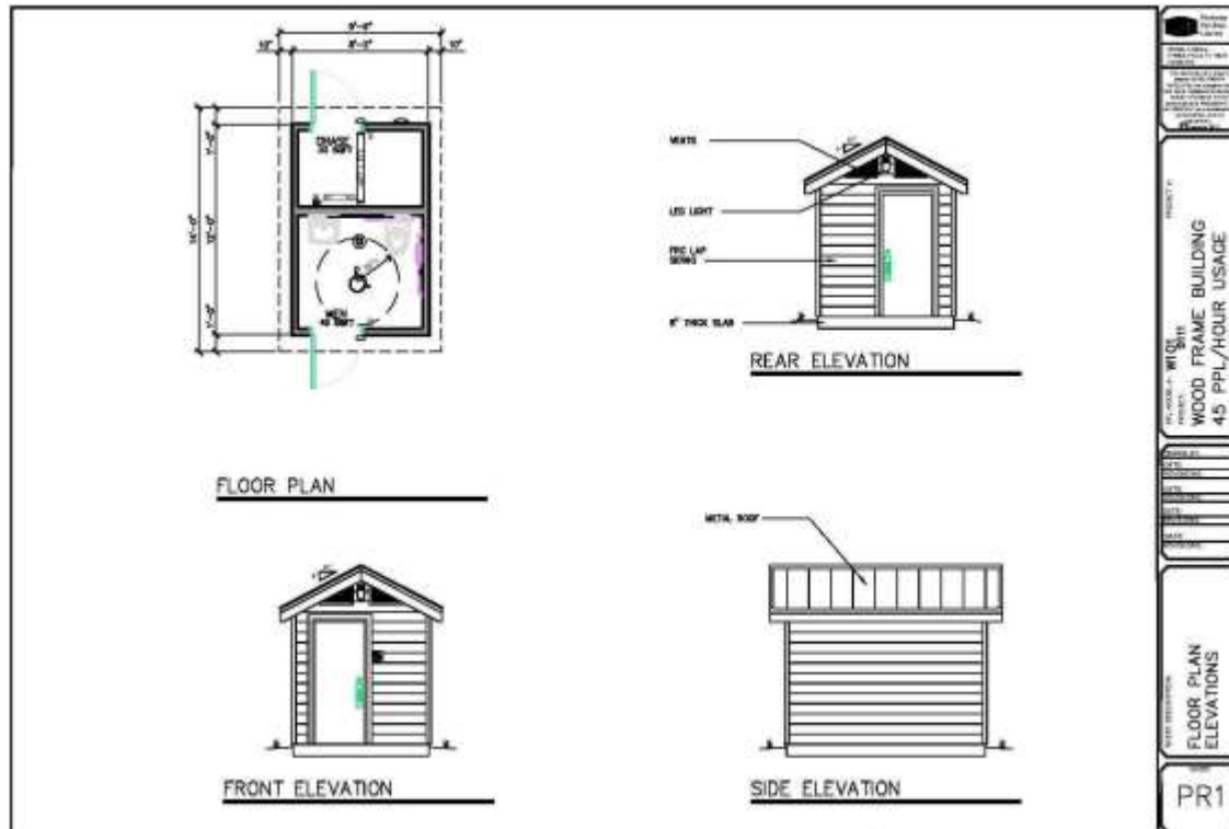
Original design without urinal
