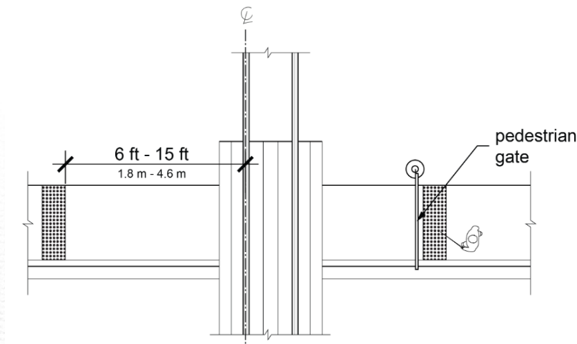
FIGURE 1. PROWAG FIGURE R305.2.5 PEDESTRIAN AT-GRADE RAIL CROSSINGS
