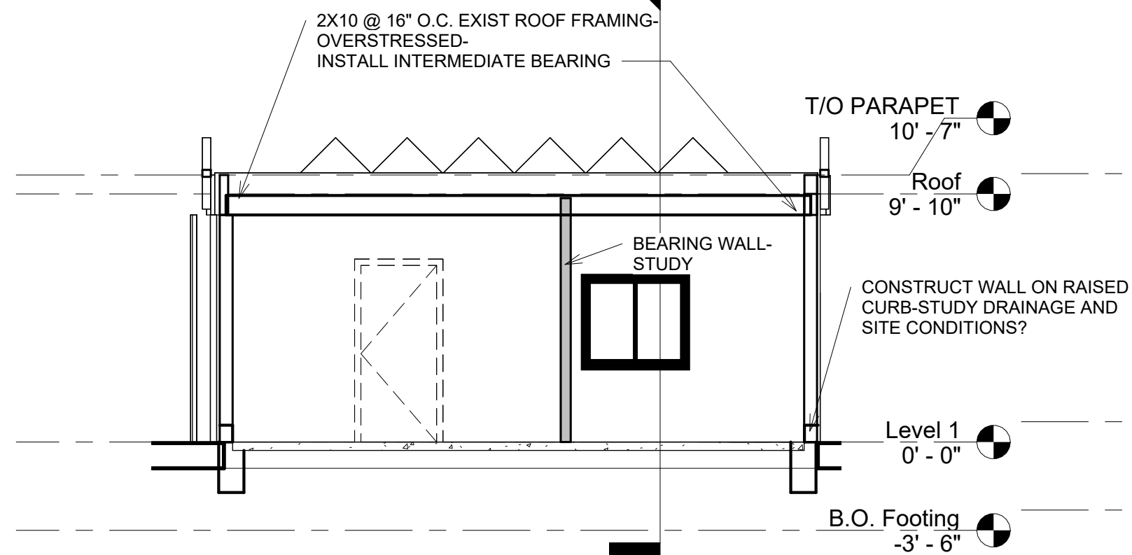
2 Section 3 3/16" = 1'-0"
