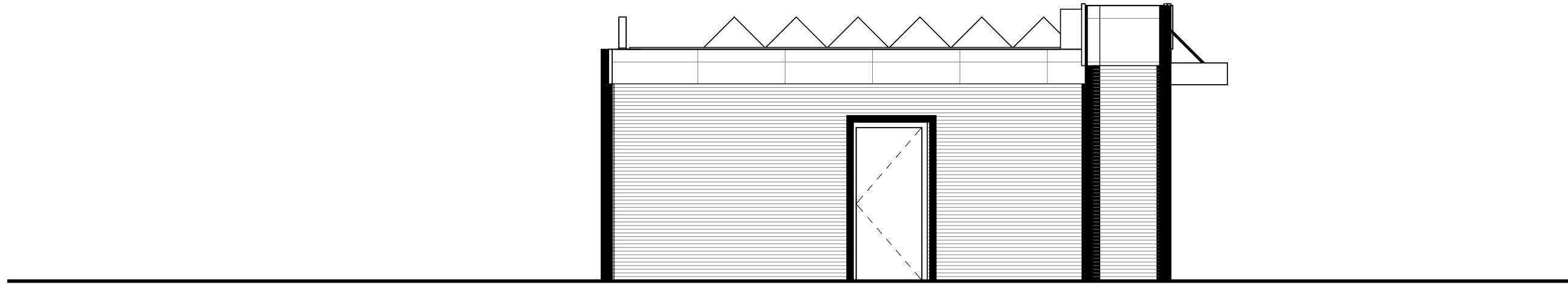
② West 3/16" = 1'-0"
