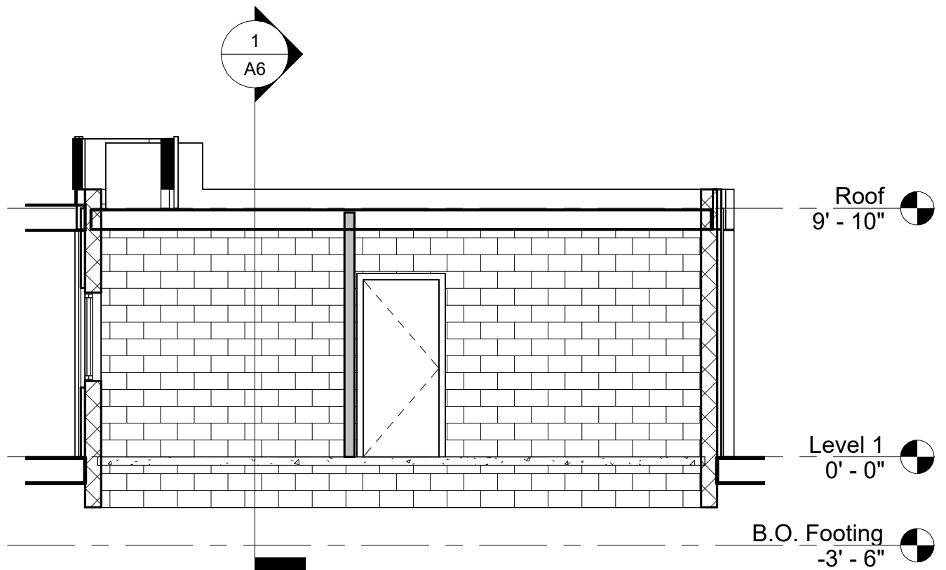
3 Section 5 3/16" = 1'-0"
