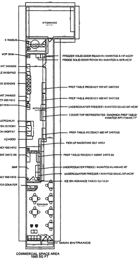
PROPOSED FLOOR PLANS 1/8" = 1'-0"
