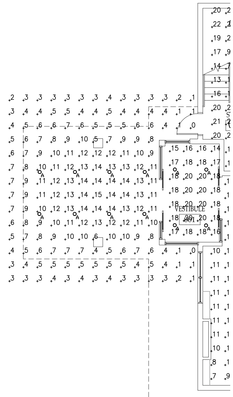
PARTIAL FIRST FLOOR LIGHTING PHOTOMETRIC PLAN
