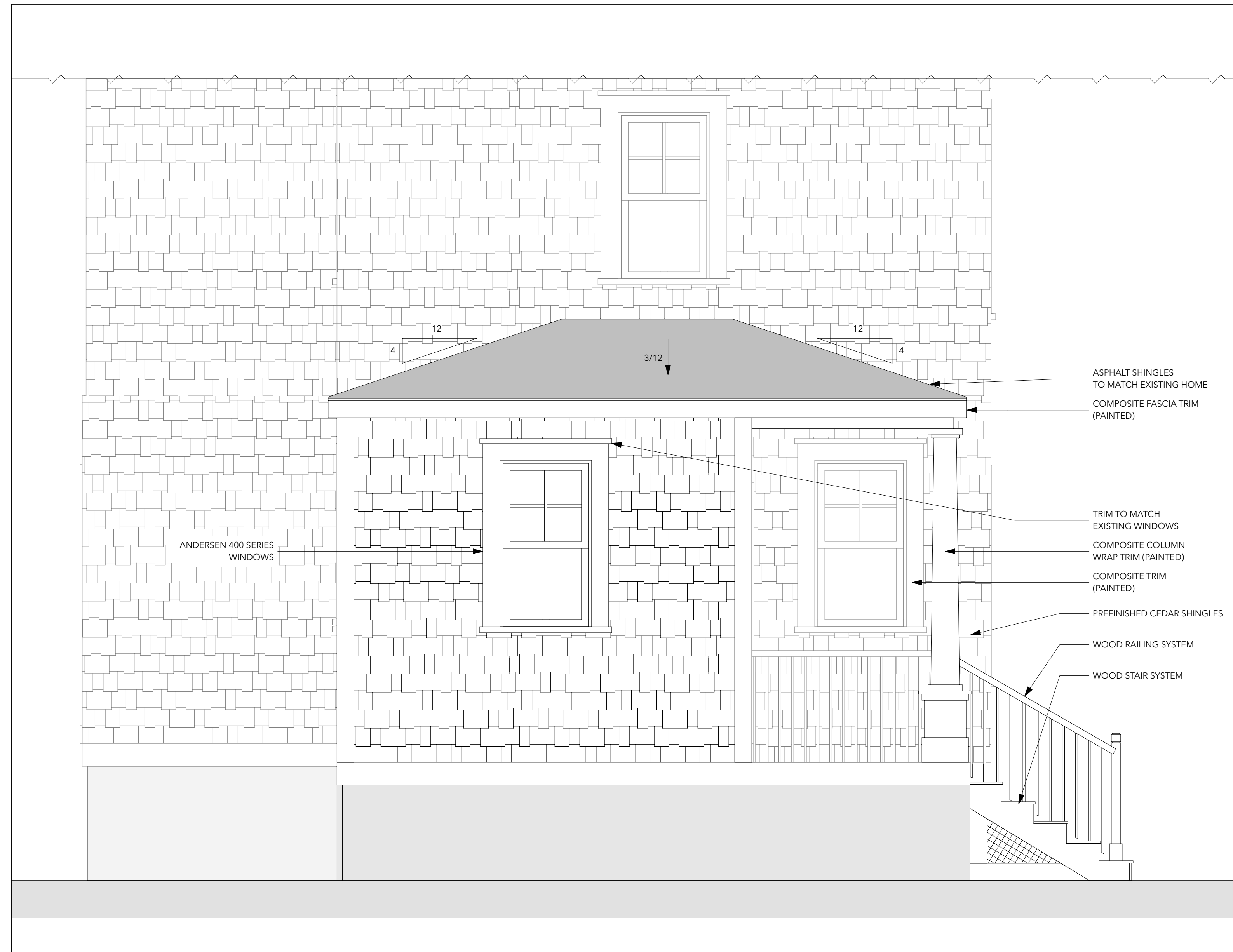
NORTH ELEVATION - PROPOSED
