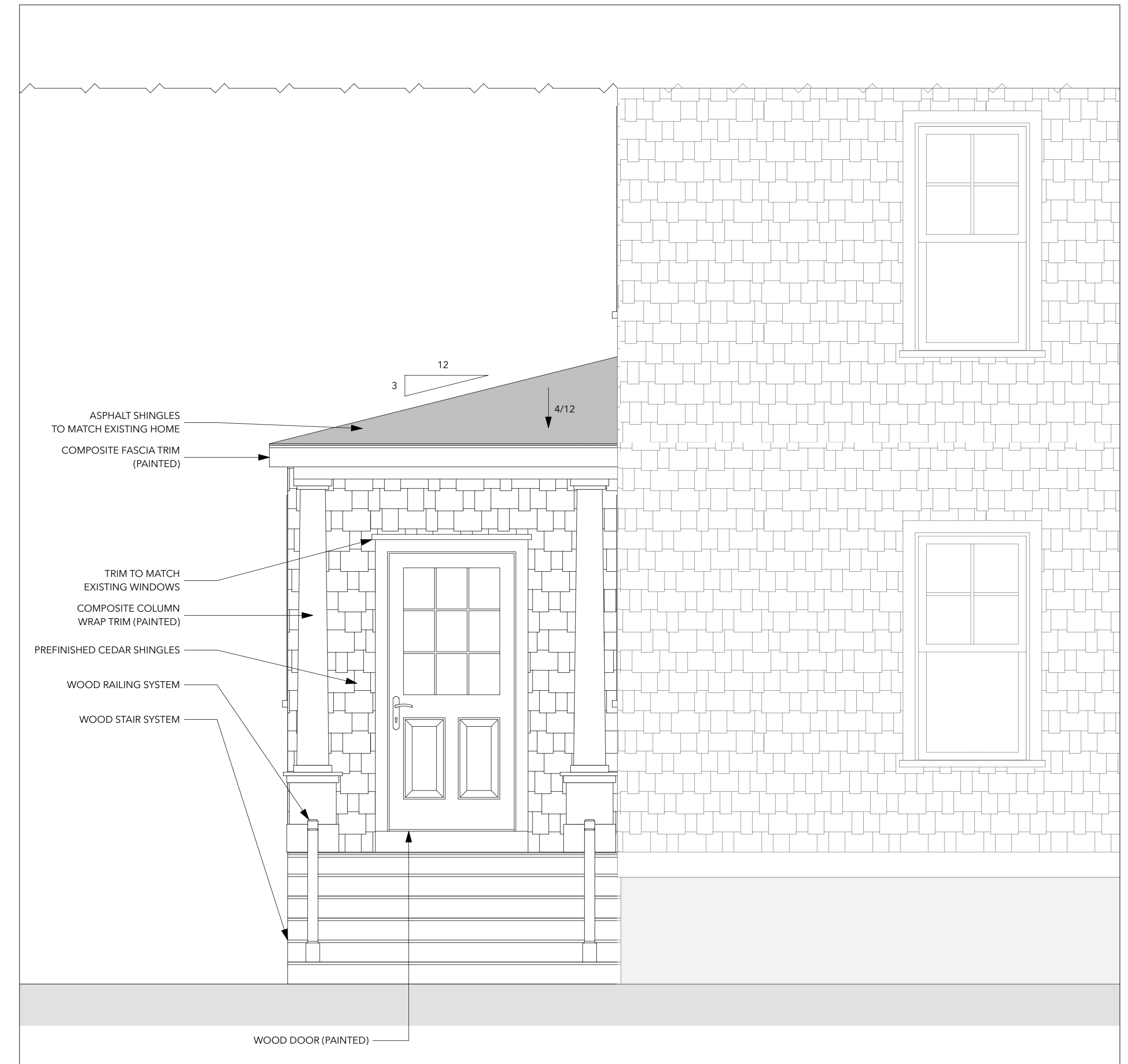
WEST ELEVATION - PROPOSED
