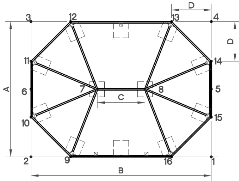
12'x16' Gazebo
