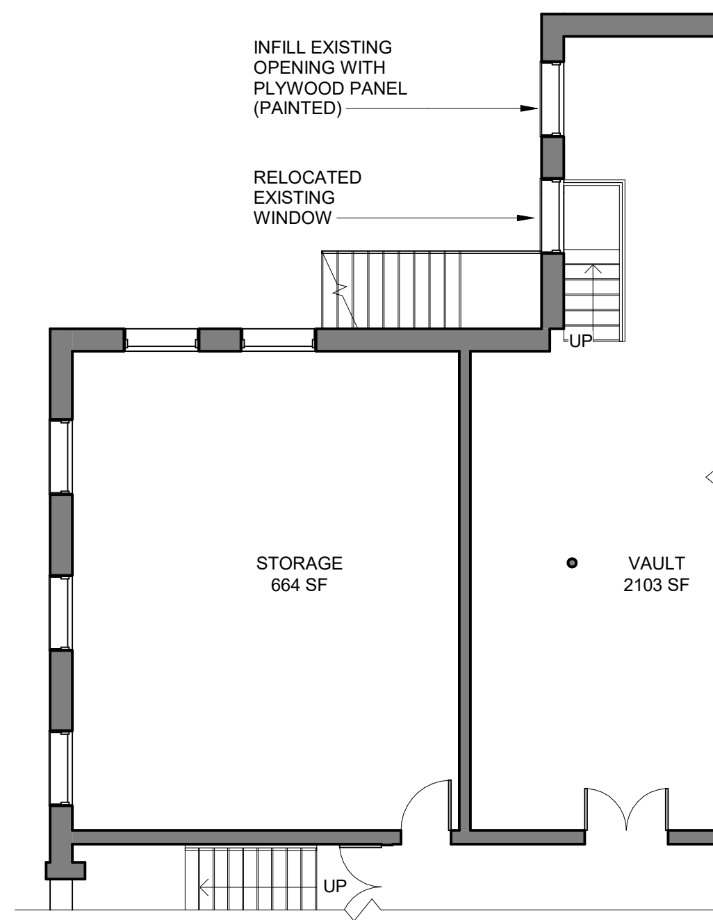
② PARTIAL BASEMENT PLAN 1/8" = 1'-0"
