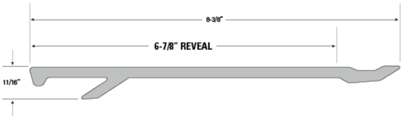
12' Plank Length Narrow 4-1/2" Lap Siding
