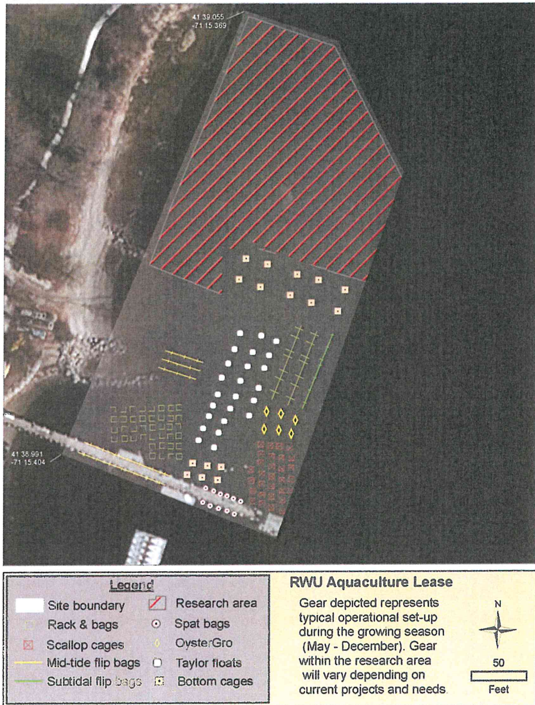
Figure 15. Plan view of the proposed aquaculture lease.
