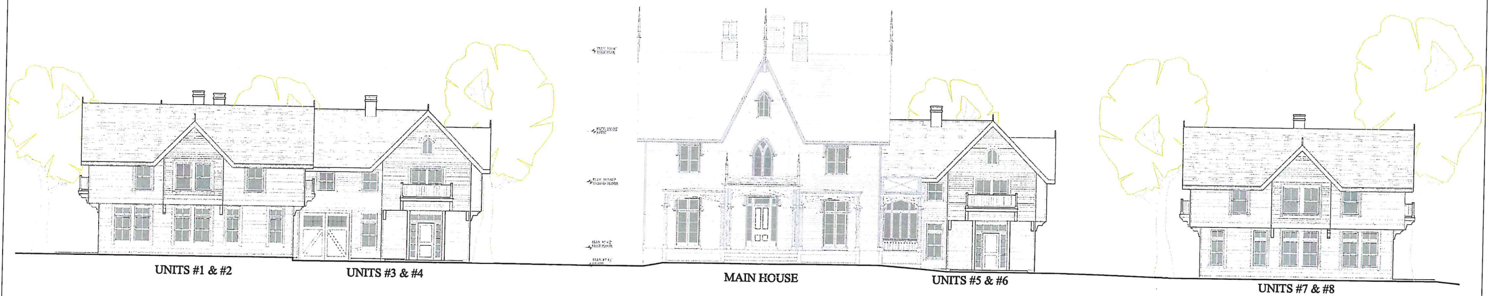
WEST ELEVATIONS SCALE: 1"=8'
