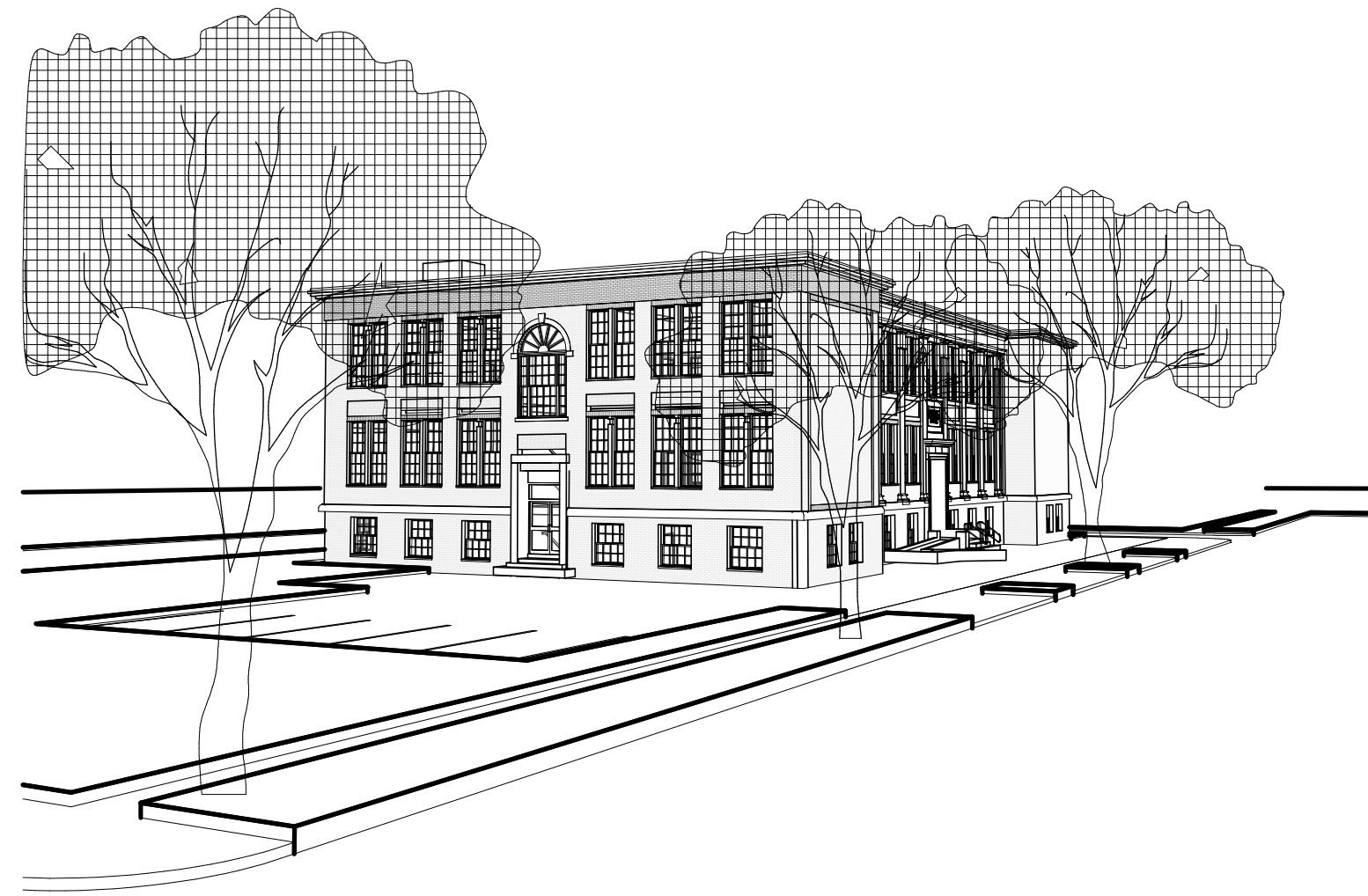
3D MODEL VIEW - NEW MECH. UNITS VISIBLE
