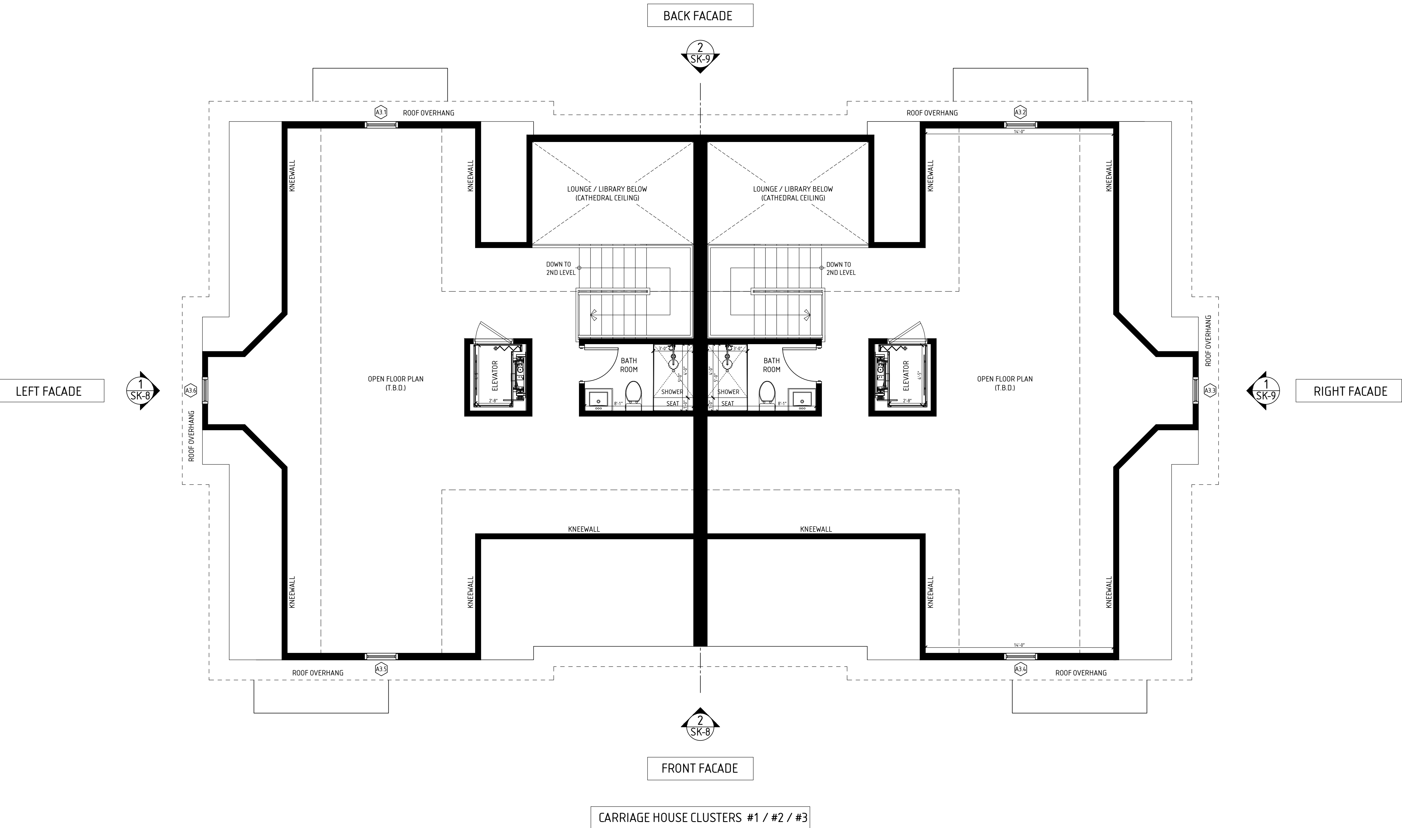
3 3RD LEVEL FLOOR PLAN - CARRIAGE HOUSE CLUSTER TYPE "A" 1200 HOPE STREET - BRISTOL - RHODE ISLAND
