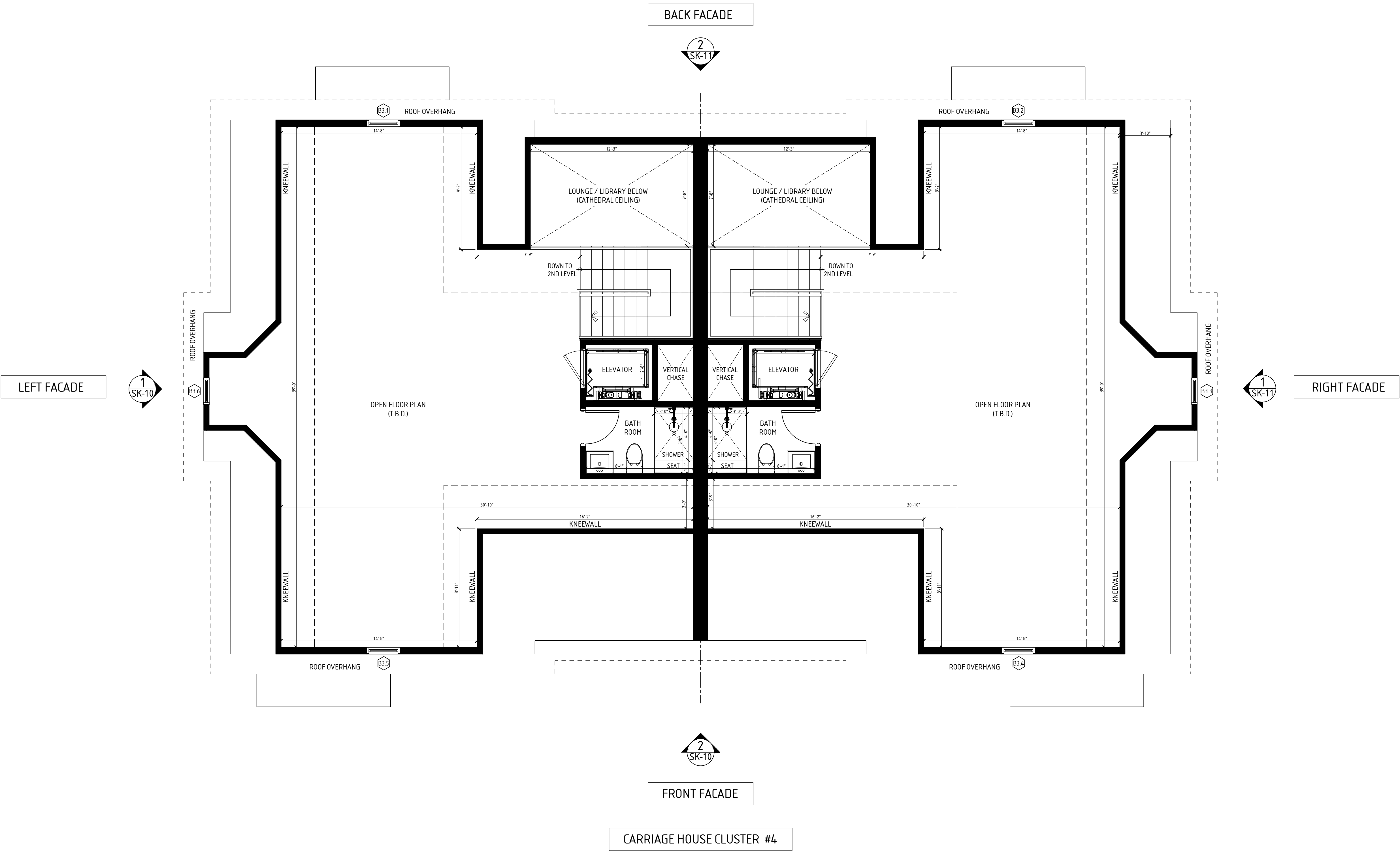
4 3RD LEVEL FLOOR PLAN - CARRIAGE HOUSE CLUSTER TYPE "B" 1200 HOPE STREET - BRISTOL - RHODE ISLAND SCALE: 1/4" = 1'-0"
