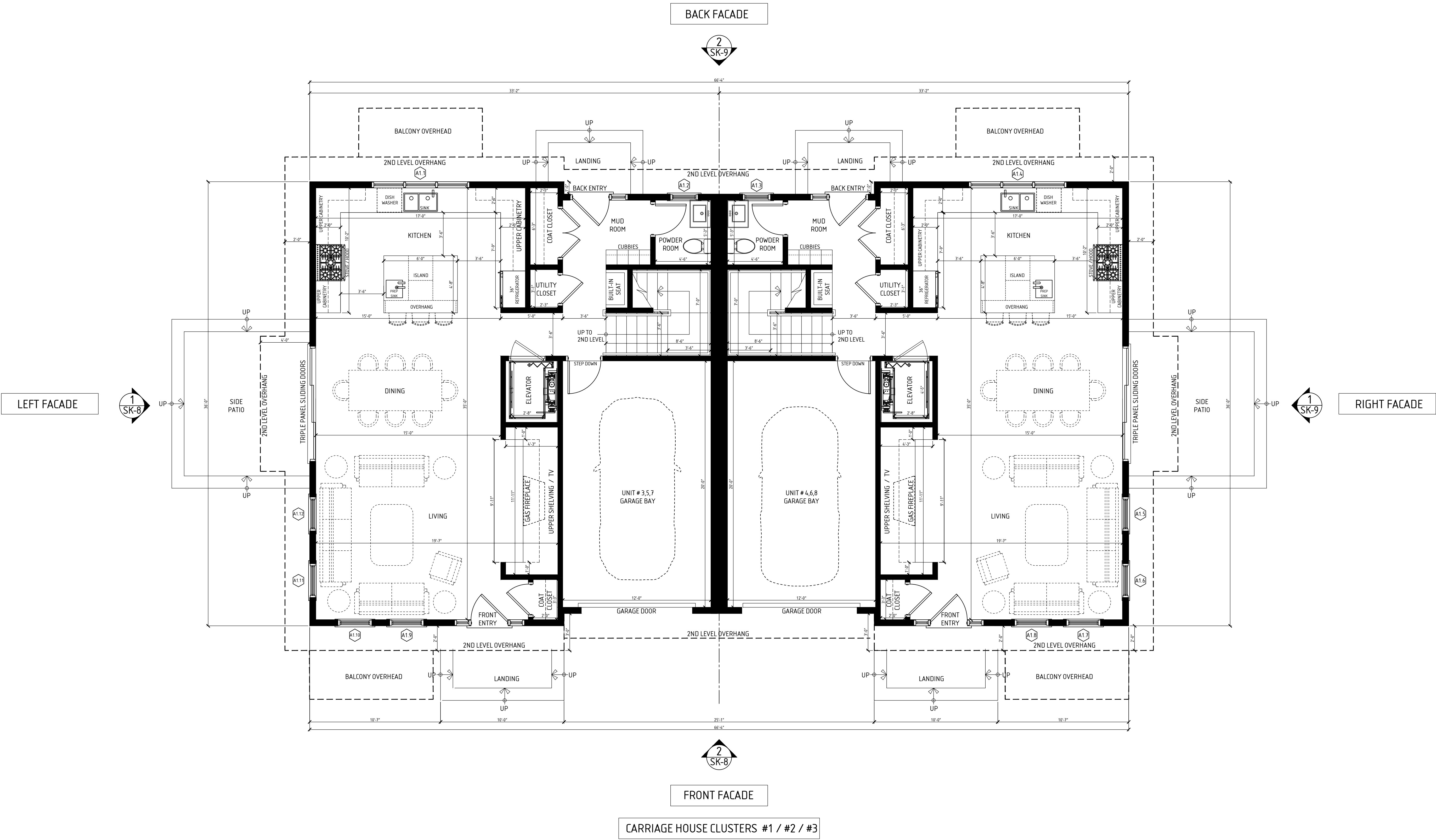
1 1ST LEVEL FLOOR PLAN - CARRIAGE HOUSE CLUSTER TYPE "A" 1200 HOPE STREET - BRISTOL - RHODE ISLAND
