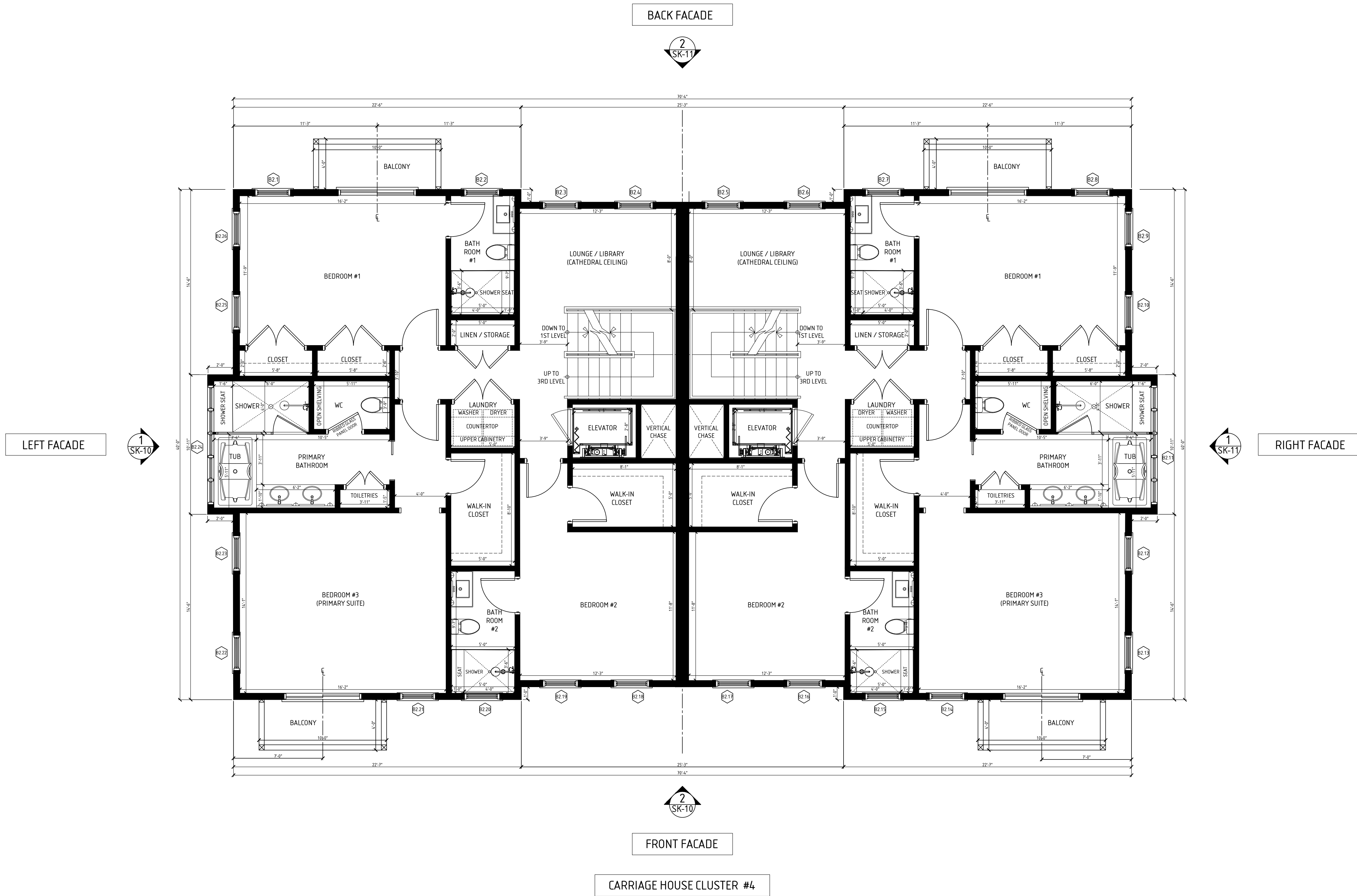
3 2ND LEVEL FLOOR PLAN - CARRIAGE HOUSE CLUSTER TYPE "B" 1200 HOPE STREET - BRISTOL - RHODE ISLAND SCALE: 1/4" = 1'-0"
