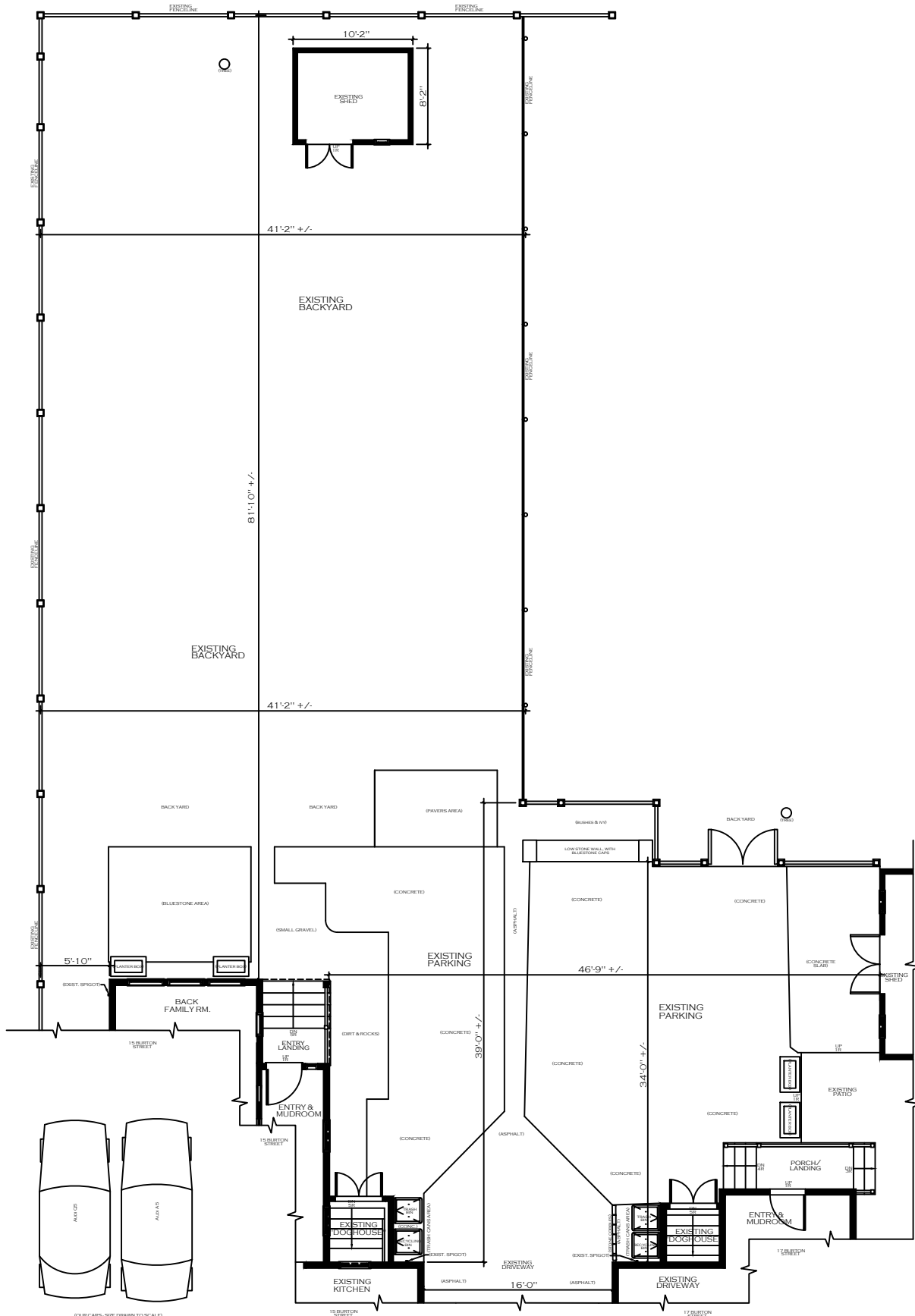
EXISTING CONDITIONS: CAR COURT & BACKYARD PLAN SCALE: 1/4" = 1'-0" (BACKYARD PLAN for 15 BURTON ONLY)
