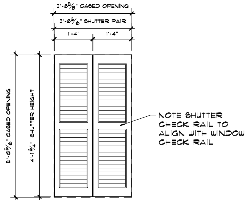
A TYPICAL EXISTING DOUBLE HUNG SHUTTER PAIR SCALE: 1/2"=1'-0"
