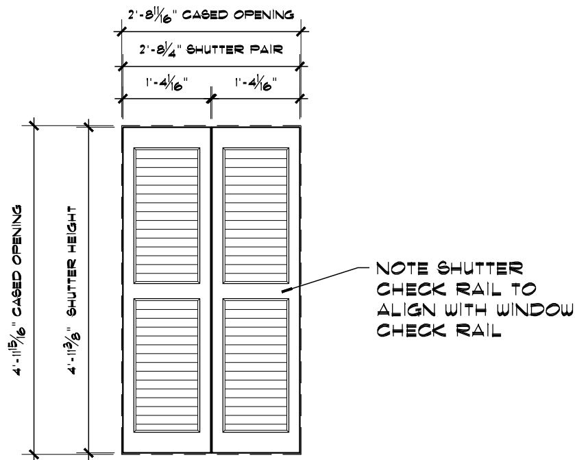
B TYPICAL NEW DOUBLE HUNG SHUTTER PAIR SCALE: 1/2"=1'-0"
